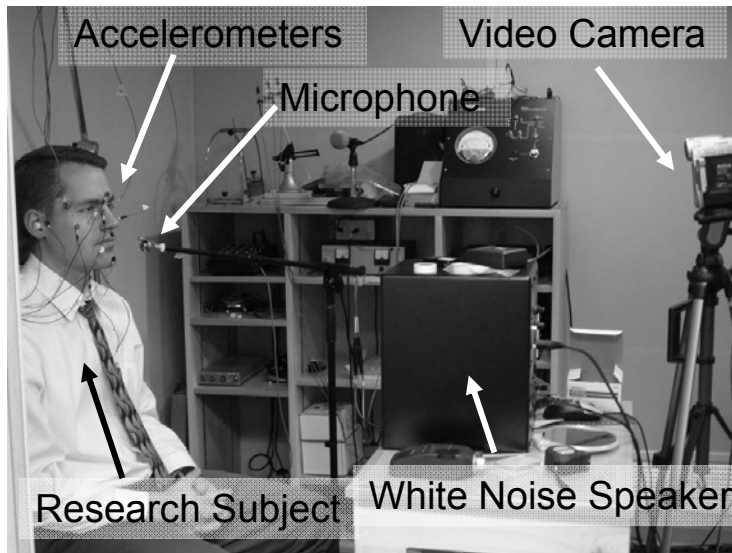
Figure A-1 Sound booth testing setup.
