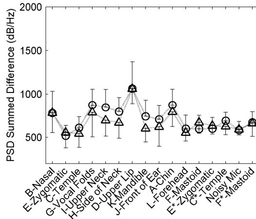
Figure 4-2 Sound /f/ normalized PSD SD for sound production with background noise. ○: Male speakers; △: Female speakers.
