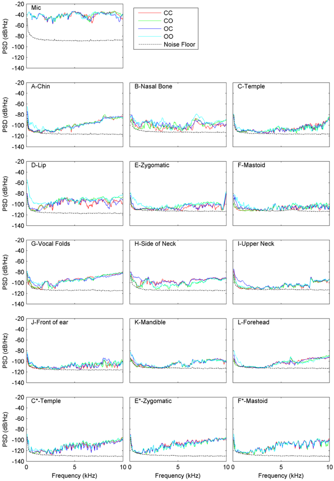
Figure 4-3 PSD plots for each location without phonation in the presence of 95 dB background noise for one male subject.
