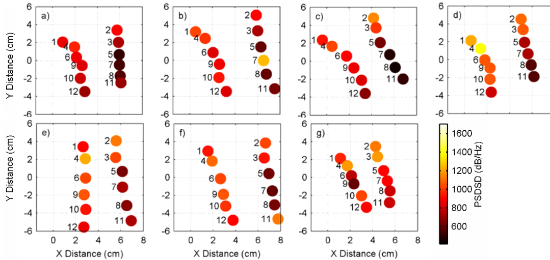
Figure 6-10 Sound /f/ neck location PSD SD plots. Female subjects a) 26; b) 27; c) 29; d) 32; Male subjects e) 25; f) 30; g) 31.
