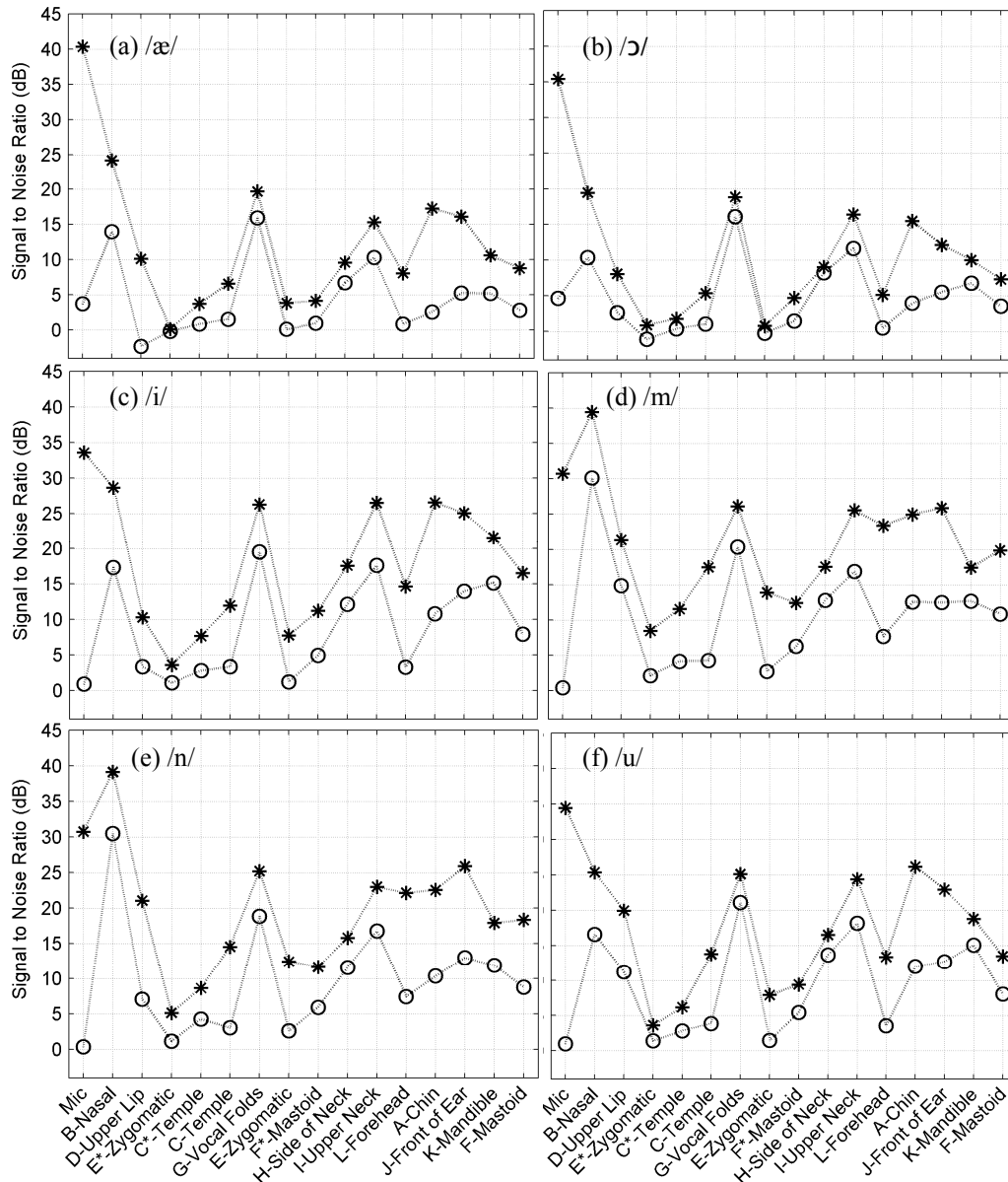
Figure 5-4 . Average SNR for female subjects. * No noise; O 95 dB background noise. a) /æ/; b) /ɔ/; c) /i/; d) /m/; e) /n/; f) /u/.
