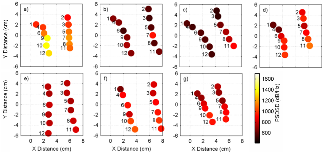
Figure 6-9 Sound /n/ neck location PSD SD plots. Female subjects a) 26; b) 27; c) 29; d) 32; Male subjects e) 25; f) 30; g) 31.
