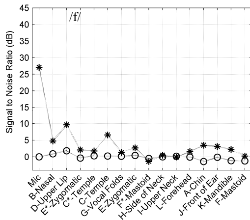
Figure 5-3 Sound /f/ average SNR for female subjects. * No noise; ○ 95 dB background noise.
