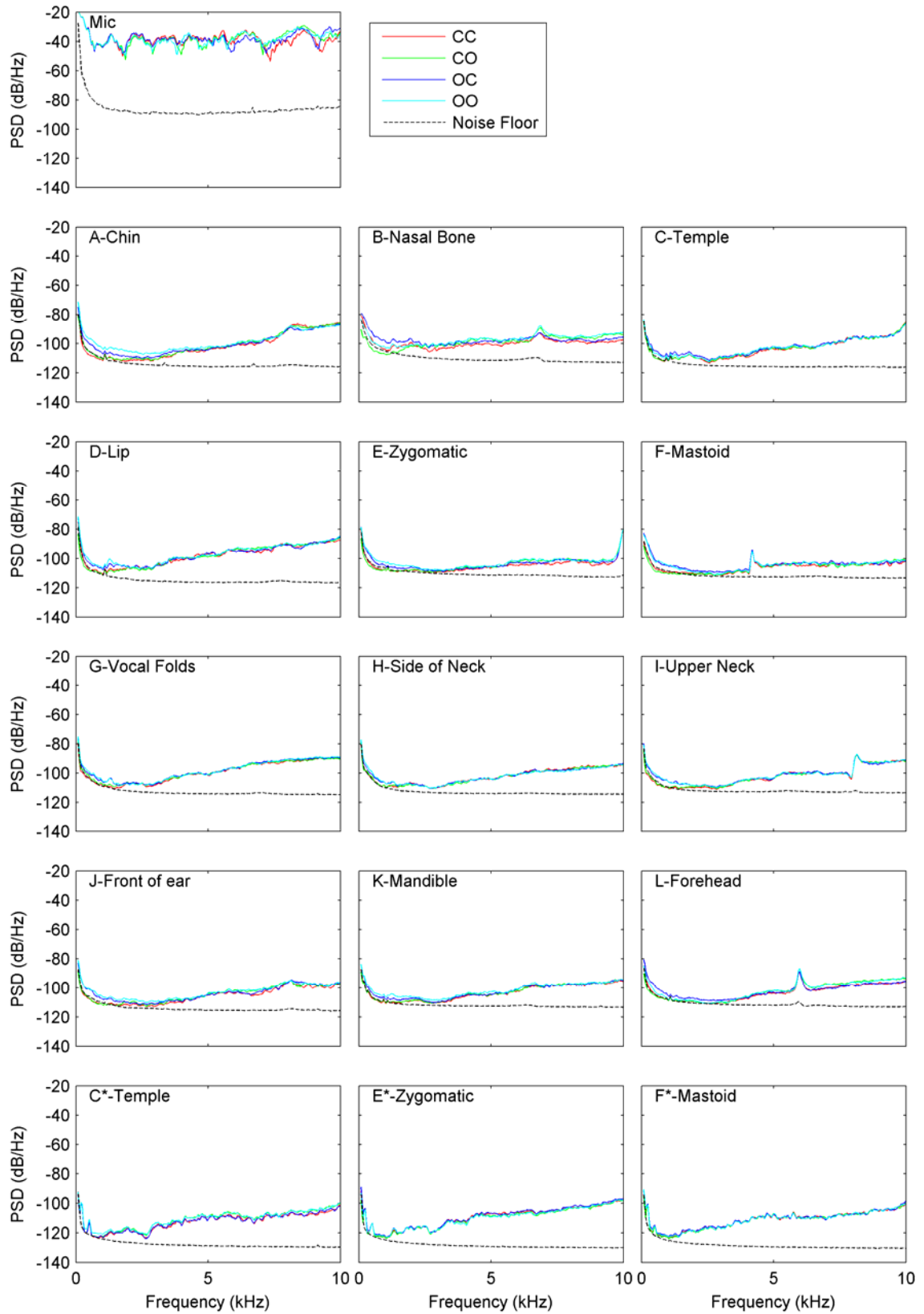
Figure 4-4 Average PSD plots for each location without phonation in the presence of 95 dB background noise.
