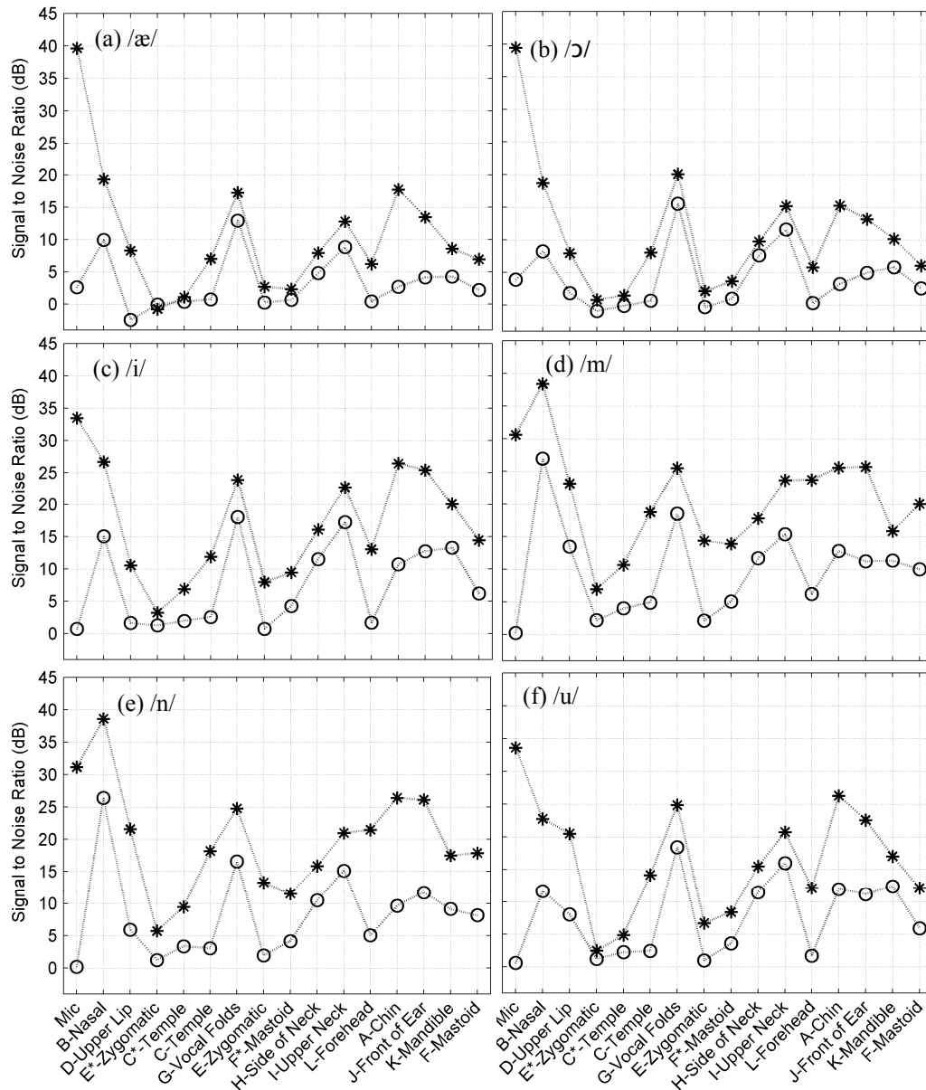
Figure 5-1. Average SNR for male subjects. * No noise; ○ 95 dB background noise. a) /æ/; b) /ɔ/; c) /i/; d) /m/; e) /n/; f) /u/.
