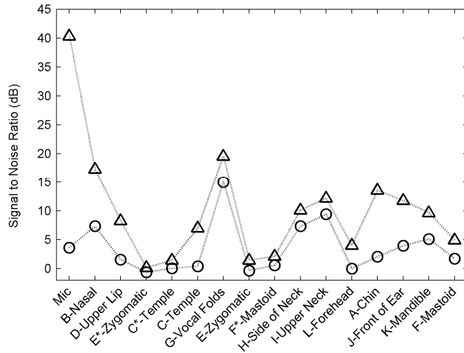
Figure 3-7 Sound /ɔ/ average SNR over all subjects. Δ: No background noise; ○: 95 dB background noise.
