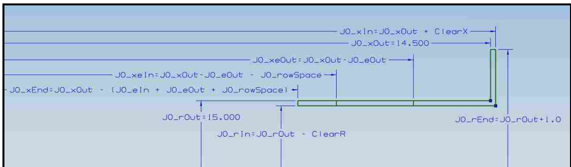
Figure 4-2: Control sketch displaying dimensions and expressions for a JointObject J0.
