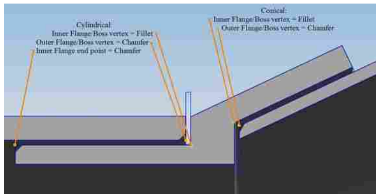
Figure 4-8: Fillet and chamfer rules
