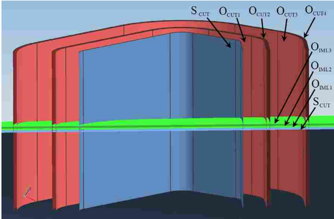
Figure 3-11: Input surfaces and offset surfaces
