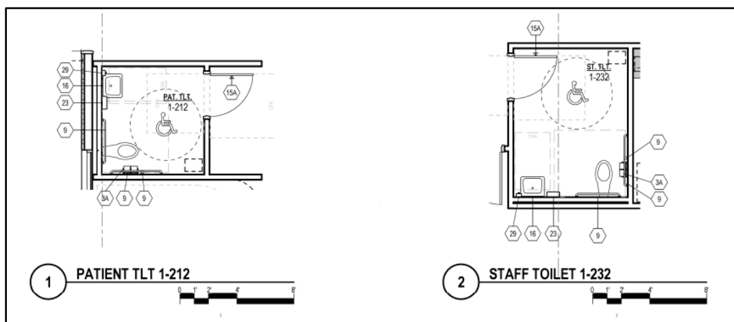
Figure 3-5: Safety Rails and Accessories in Patient and Staff Restrooms
