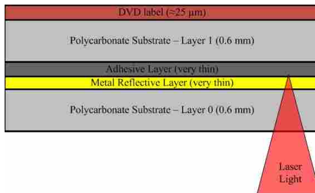
Figure 2-1: DVD Stack
