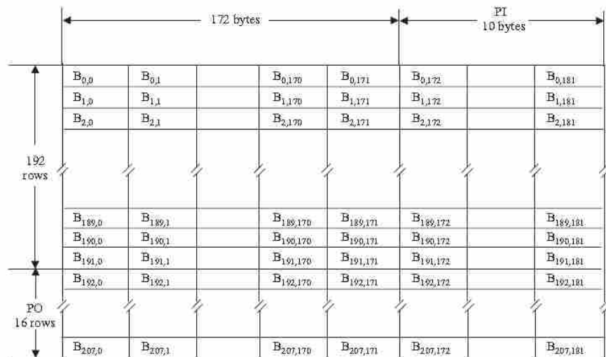
Figure 2-6: ECC Block Configuration (Ecma International 1998)
