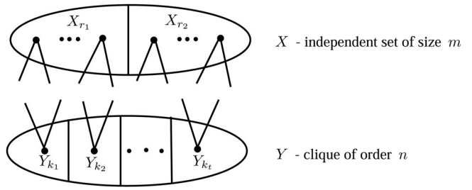
Figure 1. The split graph G .
