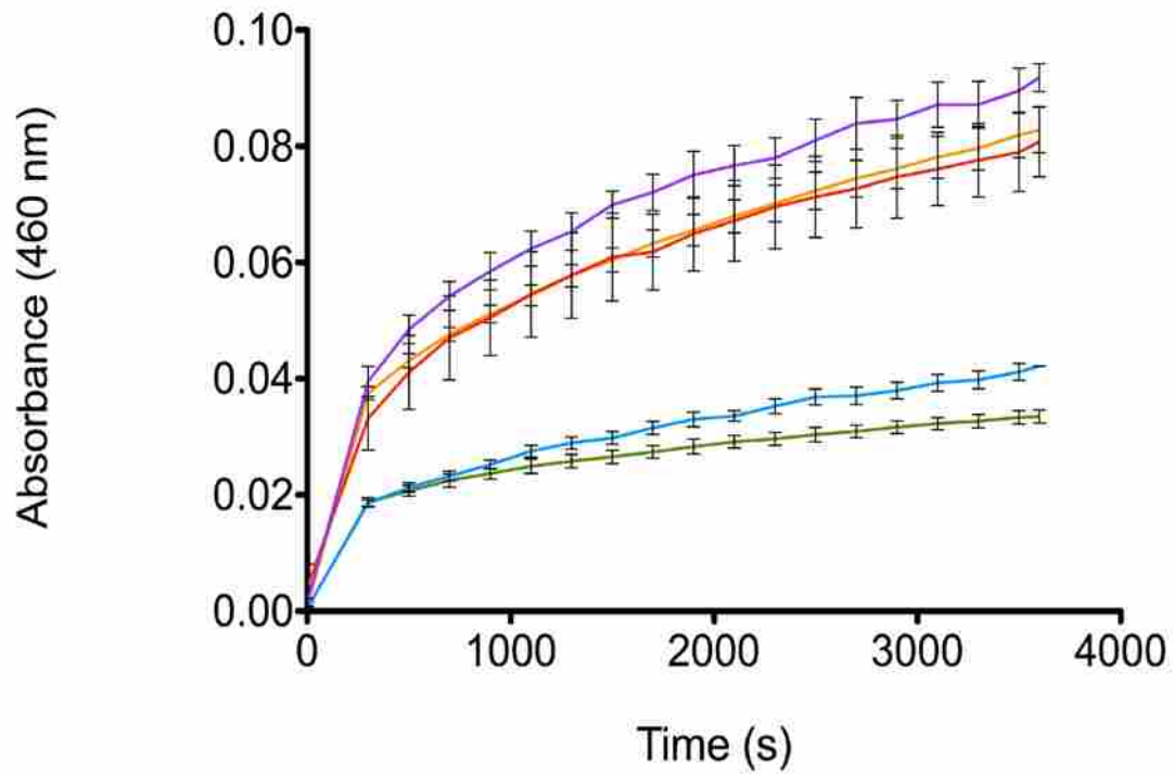
Supplemental figure 0.2 Transferrin iron loading in the presence of albumin and citrate in 10 mM phosphate. Fe 3+ was added to an apo transferrin solution with: (yellow) no other molecules, (green) 10 mM Pi, (blue) 10 mM Pi and 2 g/dL albumin, (red) 10 mM Pi with 5 g/dL albumin, (purple) 10 mM Pi with 5 g/dL albumin and 100 μM citrate).
