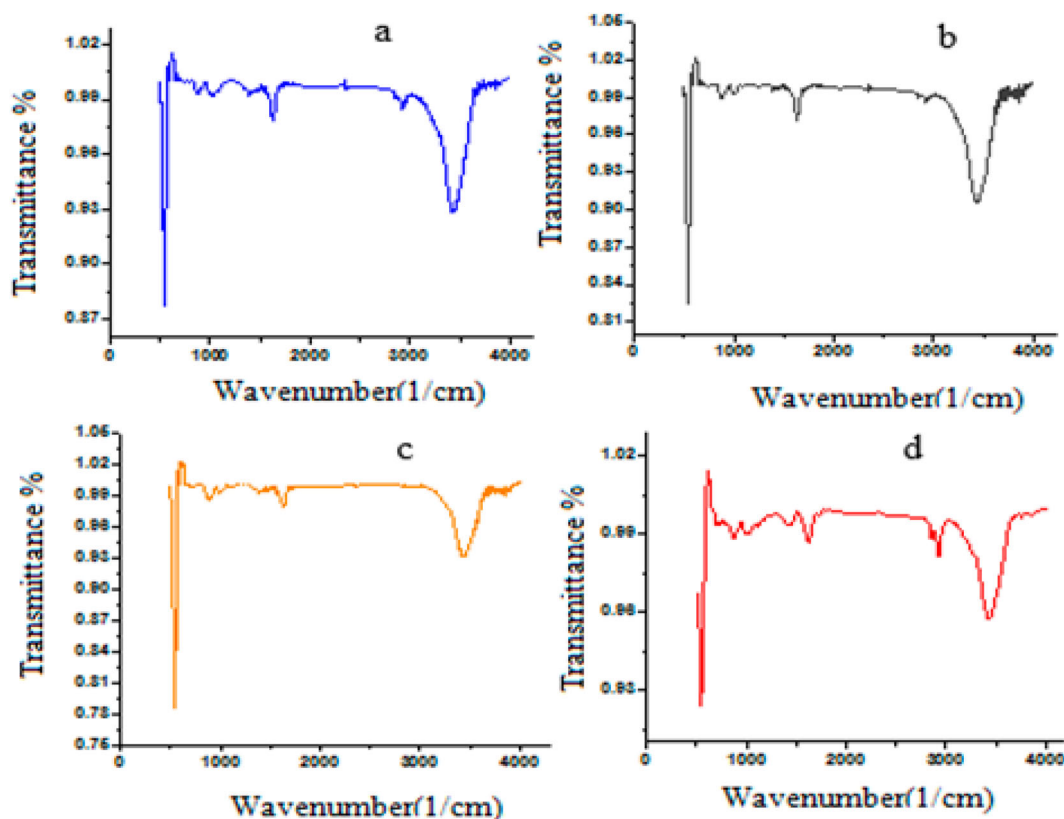
Figure 7. FTIR Diffraction pattern (a) 0.5% WO 3 doped ZnO (b) 1% WO 3 doped ZnO (c) 2% WO 3 doped ZnO and (d) undoped ZnO.
