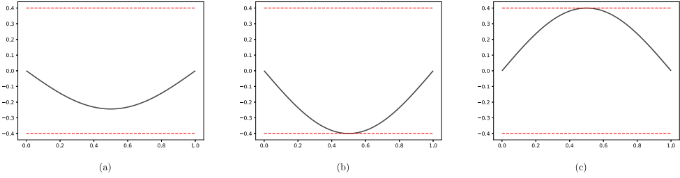
Figure 1. Solutions of the linearized beam problem (52). The dashed red lines denote the inequality constraints on the vertical displacement of the beam.
