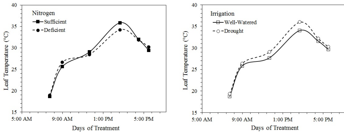
Figure 1.5 The effects of full and limited irrigation and sufficient and deficient nitrogen levels on remotely sensed maize leaf temperatures measured at six times of day on April 10, 2014 in the glasshouse (14 days since treatments began).
