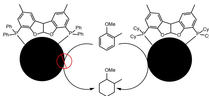
Figure 4.12 Aryl and alkyl groups containing phosphine stabilized Ru NPs for Hydrogenation
