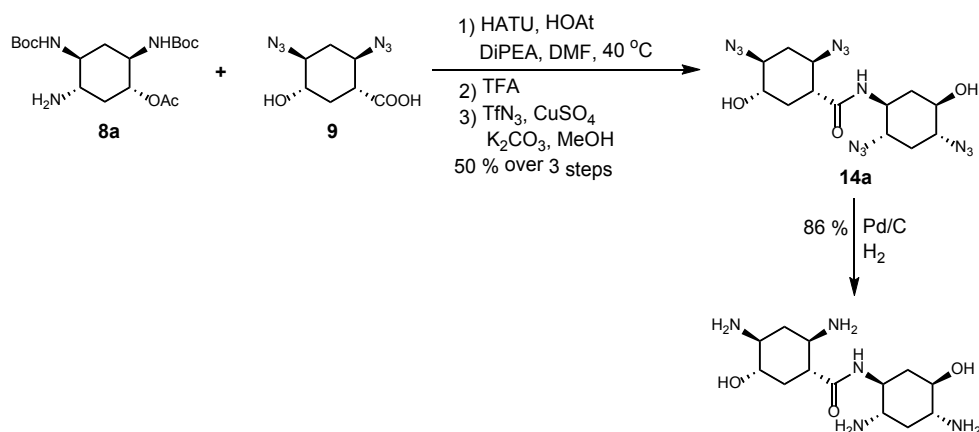
Scheme 4 Syntheses of Compound 2
