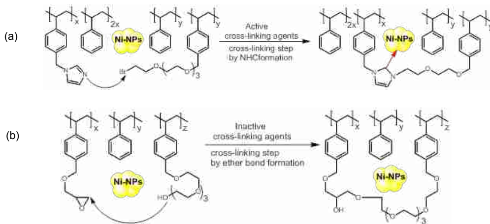
Figure 4.19 Corriu-Kumada-Tamao reaction
