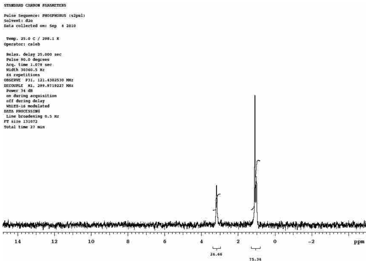
Figure 18. Phosphorous NMR of Glc-1,6P2 with glucose 1,6-bisphosphatase .
