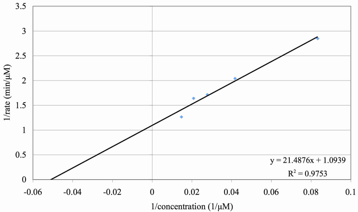
Figure 14. Lineweaver-Burk plot from which K_m and V_{max} of glucose 1,6-bisphosphatase were determined
