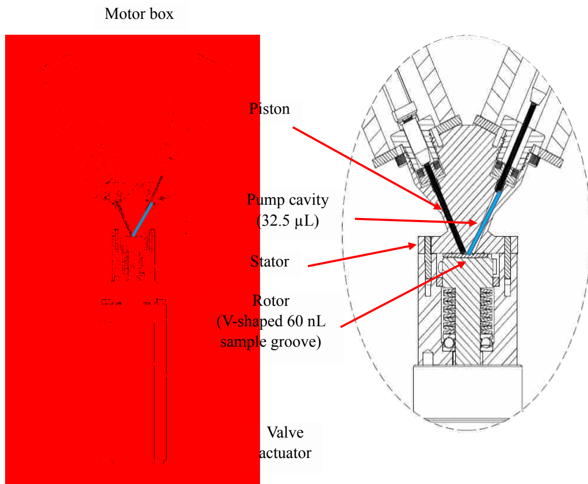
Figure 4.2 Schematic of the gradient nanoflow pumping system.
