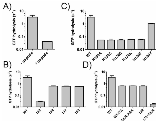
Figure 13. The SmpB C-terminal tail is critical for EF-Tu activation.
