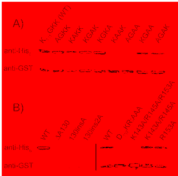
Figure 8. Mutations in the C-terminal tail impair SmpB function.
