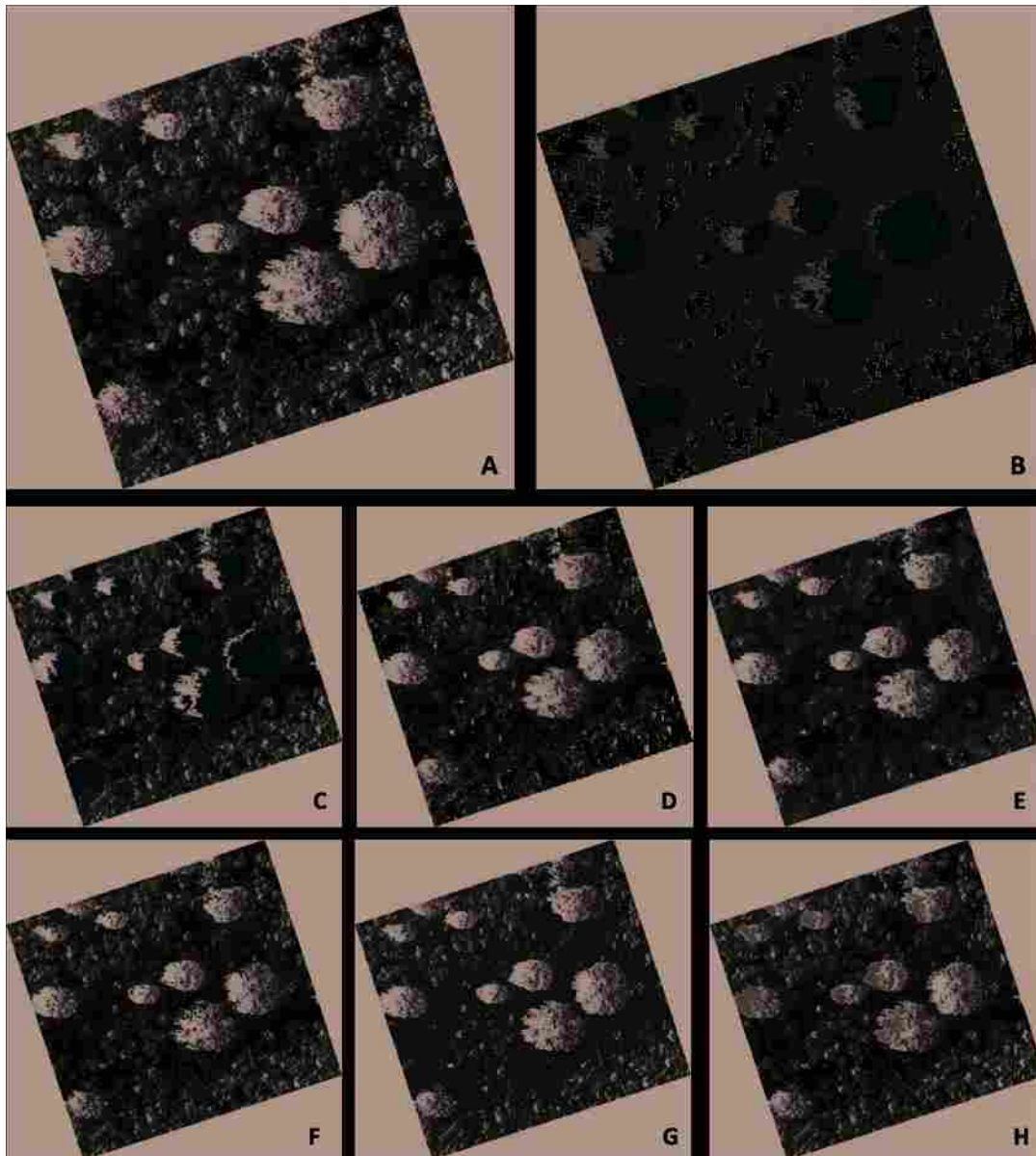
Fig. 2. Example of a juniper subplot RGB image at the onaquí Utah site (A), and the classification results using object-based image analysis (B). Individual land cover classification colors are shown that represent live trees (C; green), shrubs (D, blue), perennial herbaceous vegetation (E, orange), litter (F, pink), bare ground (G, yellow), and shadows (H, gray).
