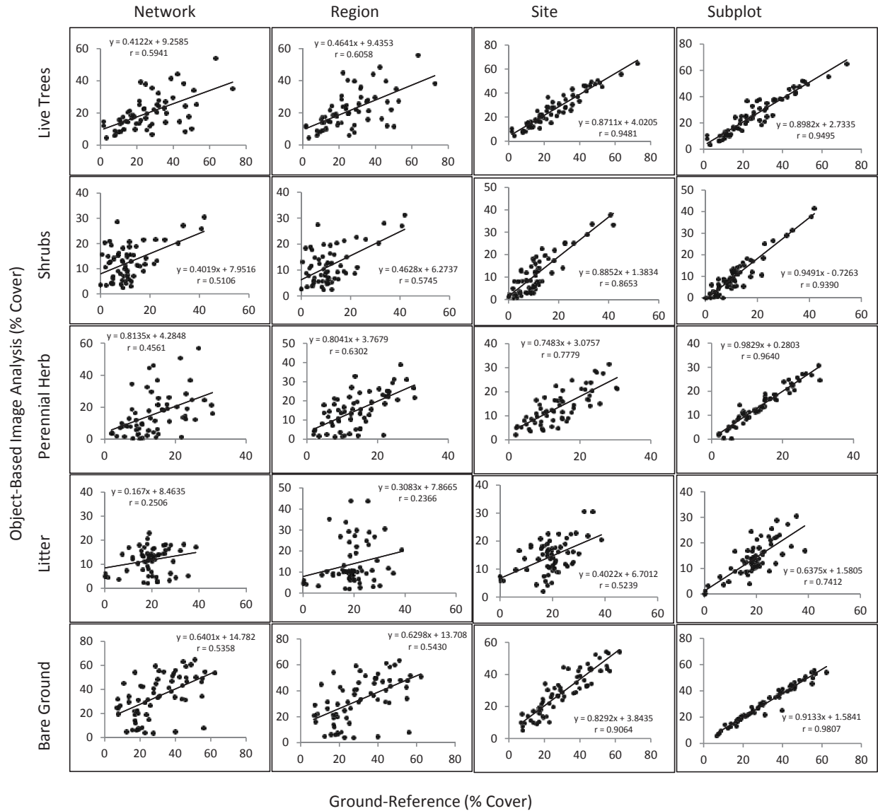
Figure 2. Regressions of percent cover estimates from an object-based image analysis (y-axis) on ground-measurements (x-axis) using subplots across all study sites (N = 65). Each row represents a land cover class (live trees, shrubs, perennial herb = perennial herbaceous vegetation, litter, and bare ground). Columns represent each spatial scale rule-set (network, region, site, and subplot) used to evaluate land cover classifications.
