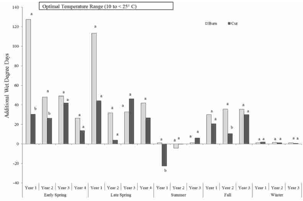
Figure 1-8. Seasonal additional wet degree days by treatment for non-optimal (top) and optimal (bottom) temperature ranges. Comparisons are within year.
