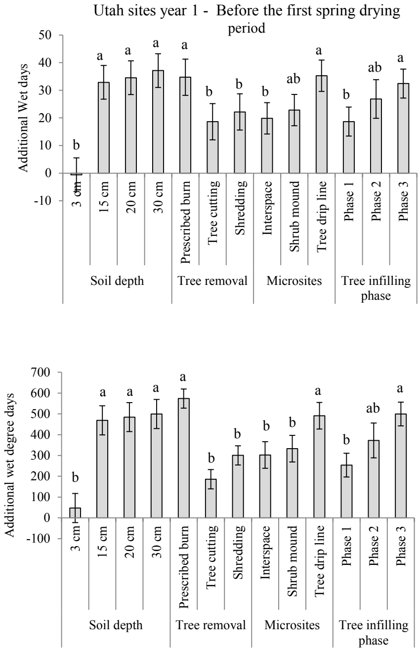
Figure 3-9. Additional wet days (top) and wet degree days (bottom) for soil depth, tree removal methods, microsites, and tree infilling phases the first year after tree reduction. Factors were separately analyzed and different letters indicate significant differences between soil depths for that year ( P < 0.05 ).
