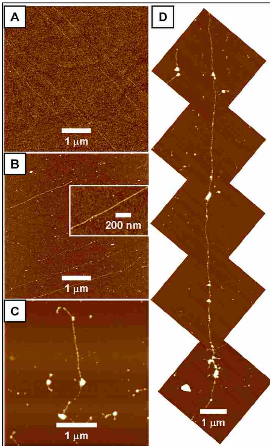
Figure 4.1. Tapping mode AFM height images of the synthesis of DNA-templated nickel. (A) Surface-aligned \lambda DNA molecules; Z scale is 3 nm. (B) DNA treated with \text{Ni}^{2+} and rinsed with ethanol; Z scale is 10 nm. (C-D) Linear nickel metal nanostructures made from surface DNA; Z scale is 50 nm in (C) and 100 nm in (D) .
