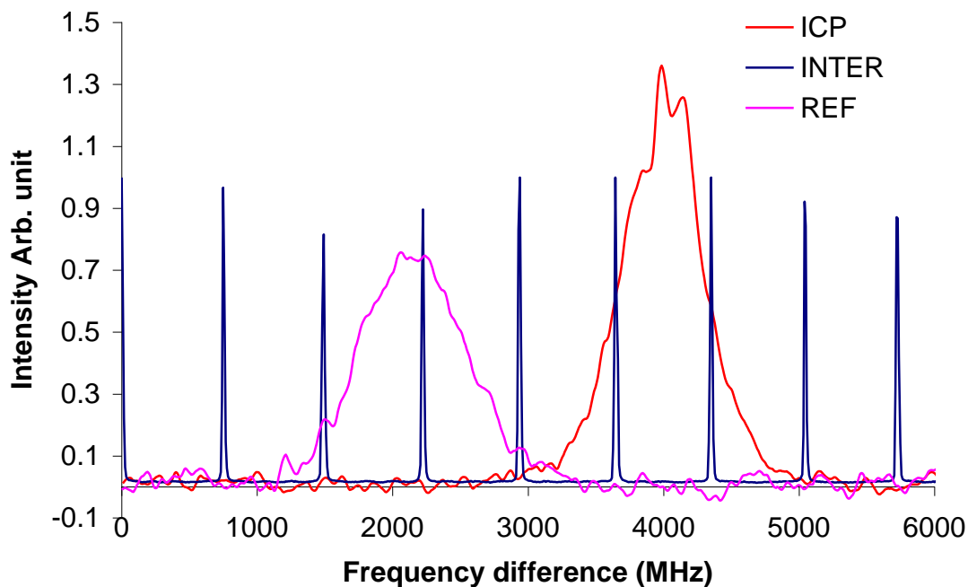
Fig 5.3 Representative signals
