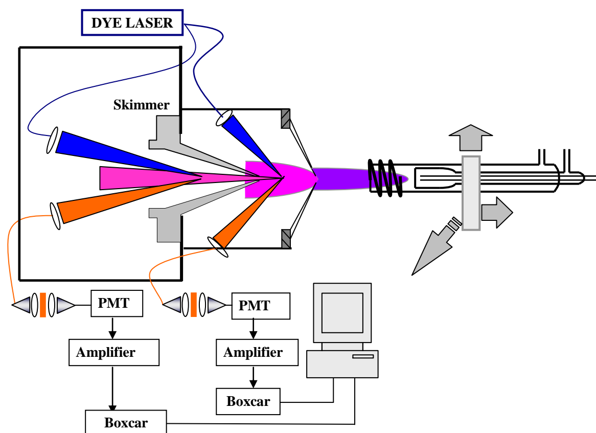
Fig 6.2 Experimental schematic
