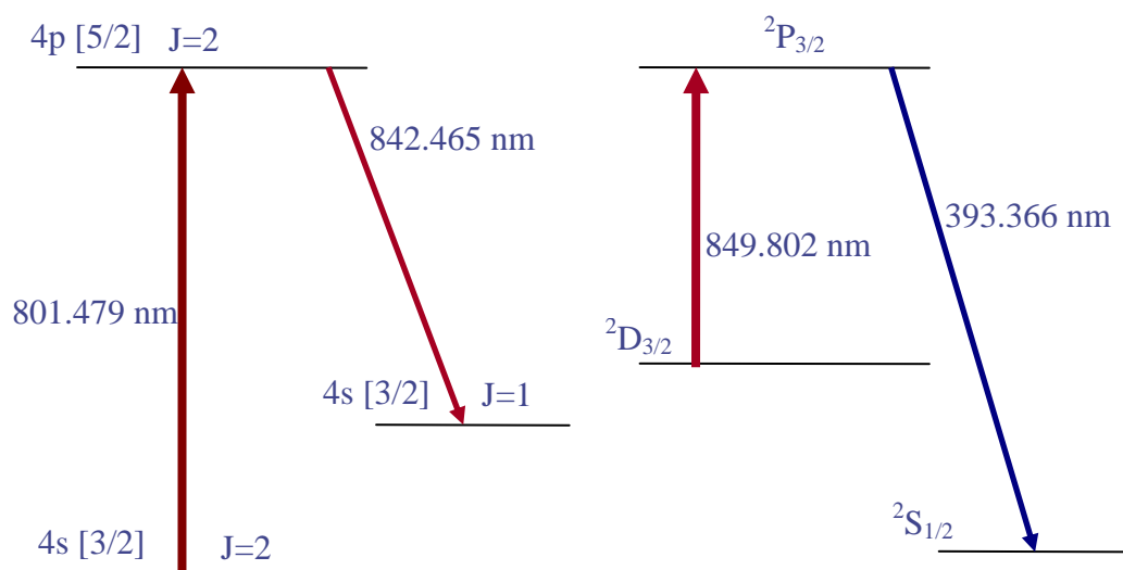
Fig 5.1 Partial Grotrian diagram for Ar I (left) and Ca II (right)
