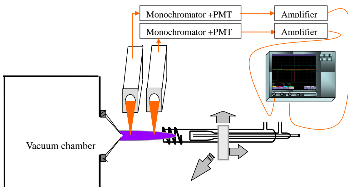
Fig 3.2 Experimental setup for particle velocity measurement inside the plasma. Two optical systems were used to collect analyte fluorescence, which is isolated by two monochromators and finally recorded by an oscilloscope
