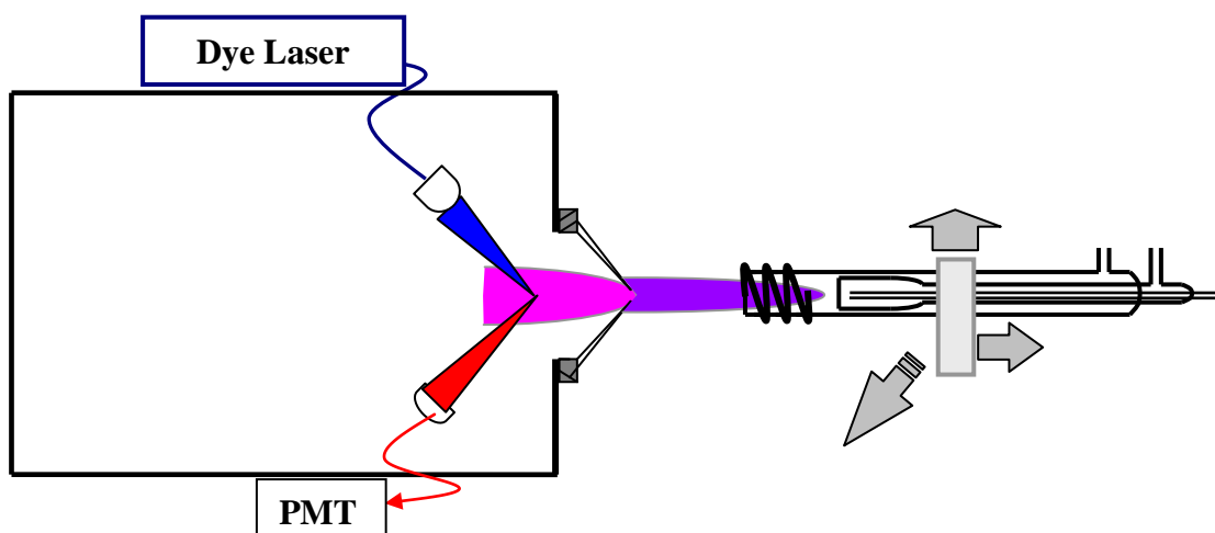
Fig 4.3 Experimental setup for fluorescence measurement 10 mm downstream from the sampling orifice
