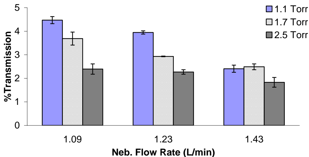
Fig 6.13 Transmission efficiencies of the skimmer cone with the variations of nebulizer flows and first vacuum stage pressures
