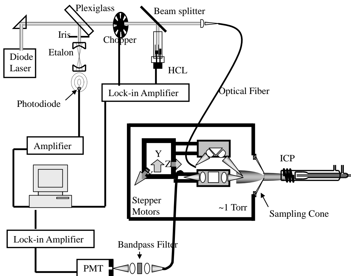
Fig 5.2 Instrument schematic
