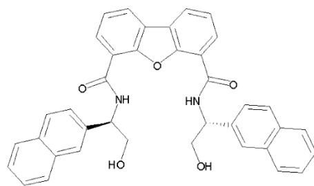
18 (CDCl 3 , 500 MHz)
