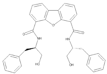
21 (500 MHz, CDCl 3 )
