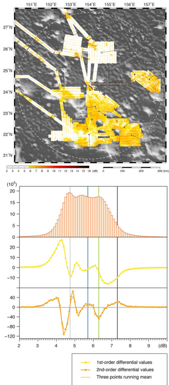
Figure 6. Integrated backscatter intensity map showing the broad distribution of ferromanganese nodules and crusts in the Japanese EEZ around Minamitorishima Island. Backscatter intensity data are established by the integration of nine datasets (MR14-E02south, MR15-E01south, MR15-E01north, MR15-E02south, MR14-E02transit, MR15-E01transit, MR15-E02transit and YK10-05SiteA and B) on the basis of the boundary intensities between the different types of seafloor facies (see the materials and methods section for details). The first- and second-order differential values are calculated from the frequency of histograms for the integrated data and are shown as a histogram. The blue, green and black vertical lines in the histogram and diagrams indicate values for the boundary intensities between different types of seafloor facies, i.e. the L–M, M–H and H–V boundaries (see the main text for details; Table 1), respectively. A grey vertical line in the histogram and diagrams indicates the value of the base intensity (see the main text for details; Table 1). Regions showing backscatter intensities lower than those observed for the L–M boundary (5.72 dB) are coloured white on the map to clearly show the broad distribution of higher intensity, which indicates the distribution of ferromanganese nodules and crusts. Uncropped integrated intensity data are shown in Figure S1. Black symbols with numeric annotation indicate observation sites using the submersible SHINKAI 6500 . The range of the map is same as that considered in Figure 1.
