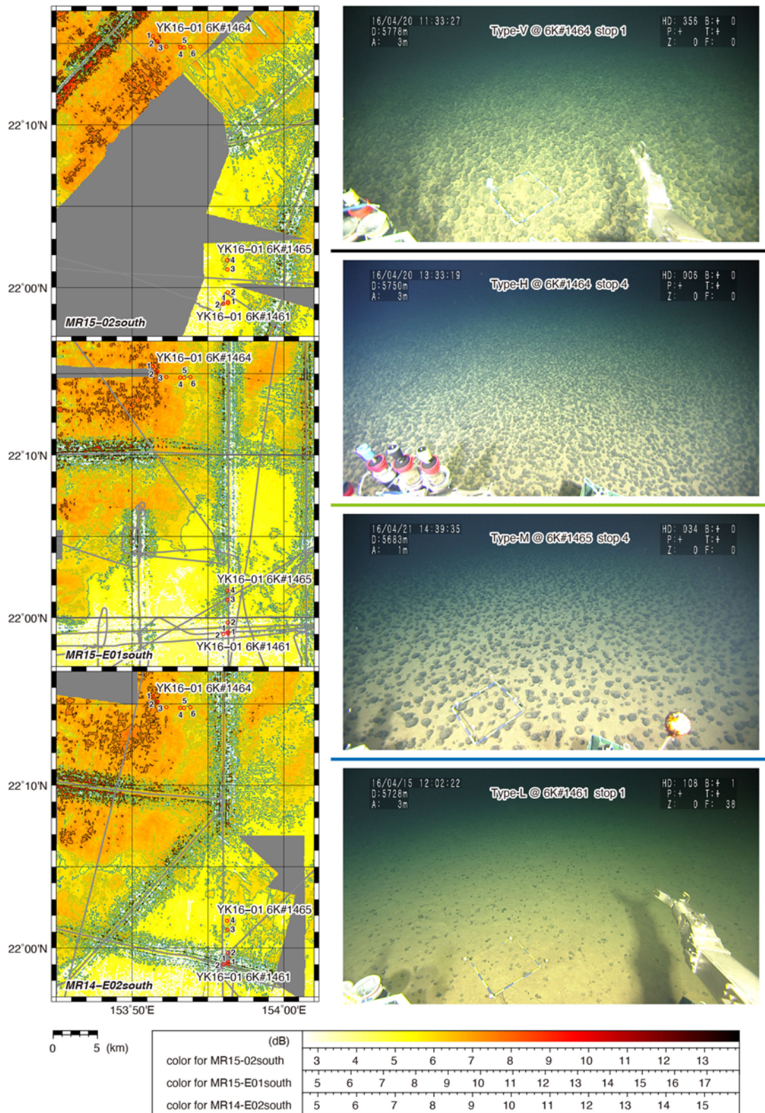
Figure 2. Map of backscatter intensity and ground-truthing observations in the type location approximately 200 km south of Minamitorishima Island. Multiple sets of backscatter intensity data (MR14-E02south, MR15-E01south and MR15-02south) are shown in the different panels on the left. The range of the map for each dataset is the same and is shown as a white box in Figures S2–S4 (supplementary material). Grey lines illustrate ship track of each cruises. Photographs on the right show the types of seafloor facies (Type-L, Type-M, Type-H and Type-V facies; see the main text for details) and are taken at stops (red circles on the map, with numeric annotation indicating stop numbers) during three dives of the submersible SHINKAI 6500 (dive Nos. 6K#1461, #1464 and #1465; see supplementary material for details). One side of the blue/yellow-banded box is 50 cm. Geographic distributions of the seafloor showing values of the boundary intensities between the different types of seafloor facies, i.e. L–M, M–H and H–V boundaries (see the main text, Figure 3 and Table 1 for details), are illustrated blue, green and black contour lines, respectively, in the intensity maps. The white contour line indicates the geographic distribution of the seafloor showing the base intensity (see the main text, Figure 3 and Table 1).
