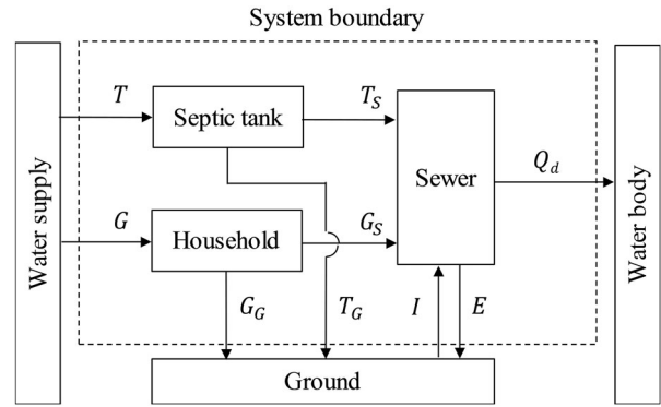
Figure 2. System boundary and components of the water balance model for the target sewer on no-rain days. T : flush toilet water, G : greywater, T_S and T_G : septic tank effluent discharged into the sewer and ground, respectively, G_S and G_G : greywater discharged into the sewer and ground, respectively, I : infiltration, E : exfiltration, and Q_d : sewage discharged from the single sewer outlet.
