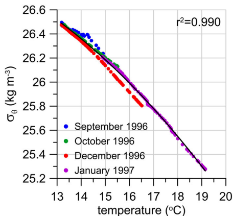
Figure 3. Density ( \sigma_\theta ) versus temperature for all CTD data collected over the four cruises at station B1. The black solid line is the 2nd order polynomial fit to the data, with a root-mean-square deviation of the data around the fit of 0.03 \text{ kg m}^{-3} .
