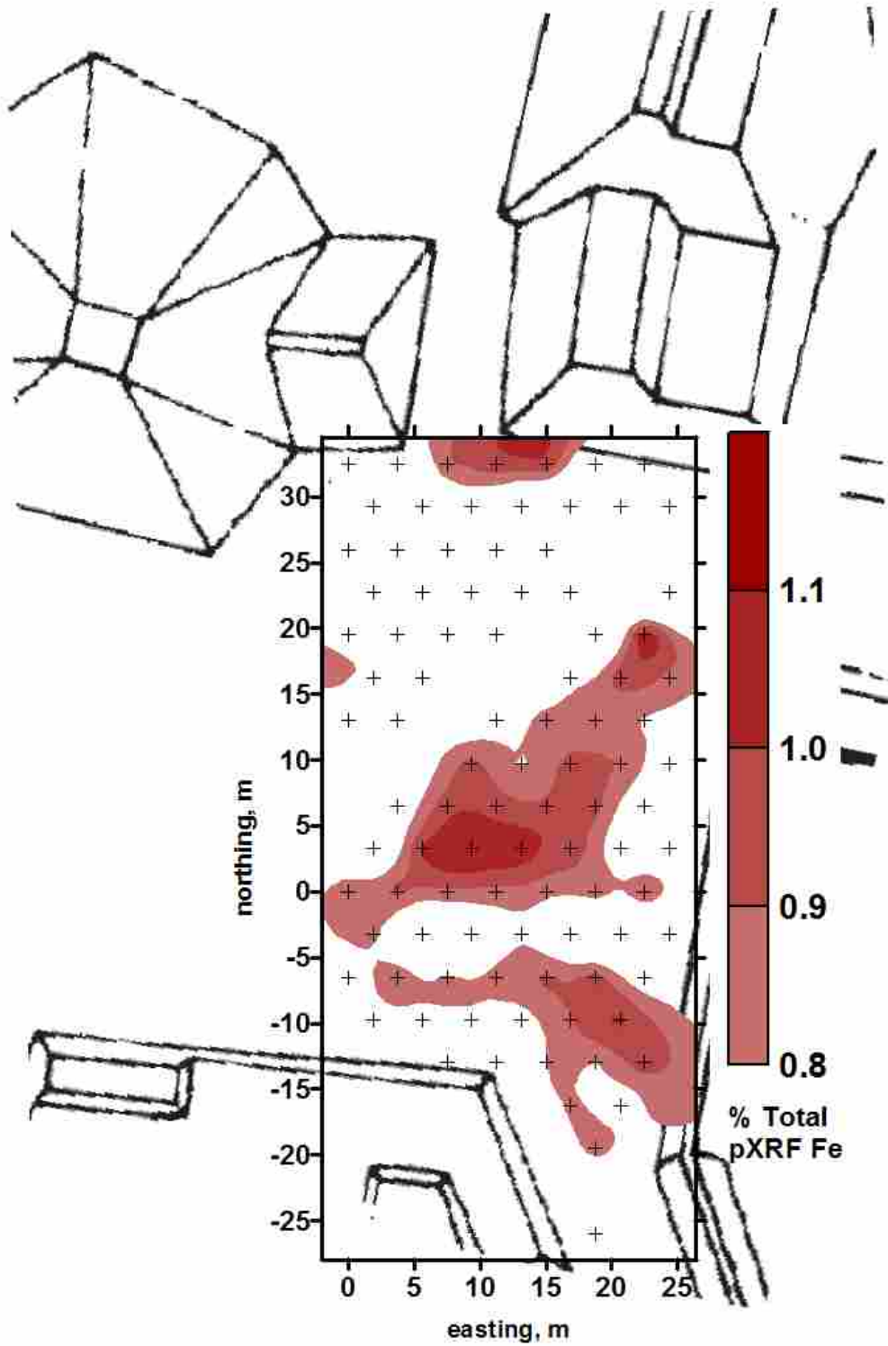
Figure 2-14. Concentration isopleths of pXRF total Fe within the sampling area near Caana.
