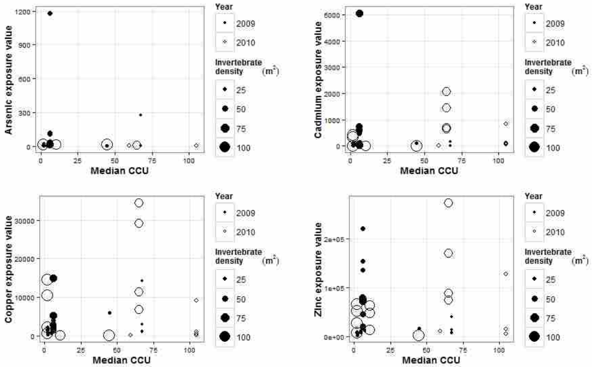
Exposure value (all taxa) vs sediment CCU (2009 & 2010)
