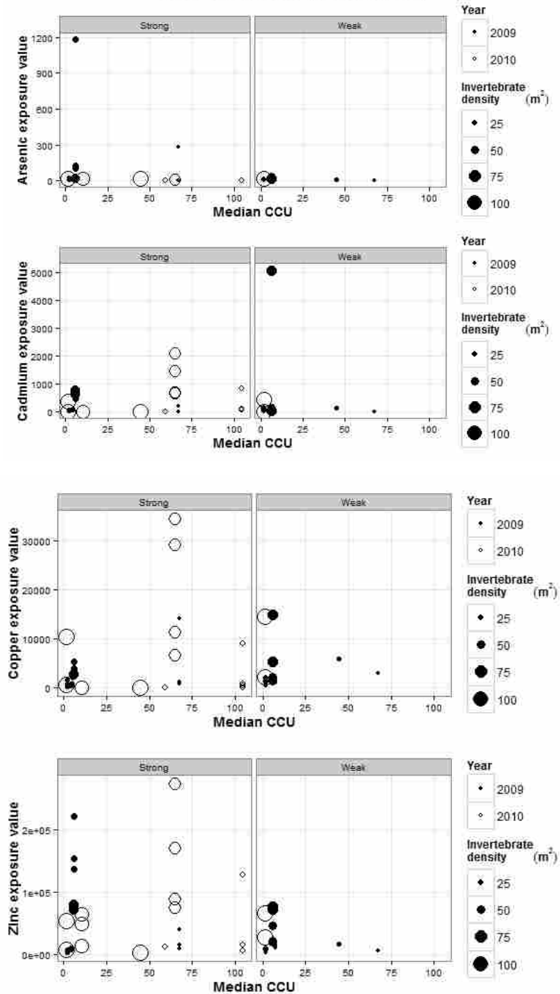
Figure 15: Exposure values for invertebrates with strong and weak propensity to drift vs. sediment contamination (CCU = cumulative criterion units) for all upper Blackfoot River sites sampled in 2009 and 2010. Point size reflects the invertebrate species' density with larger points corresponding to higher densities. Solid circles identify 2009 data and open circles identify 2010 data. Each point represents exposure values for an individual species.
