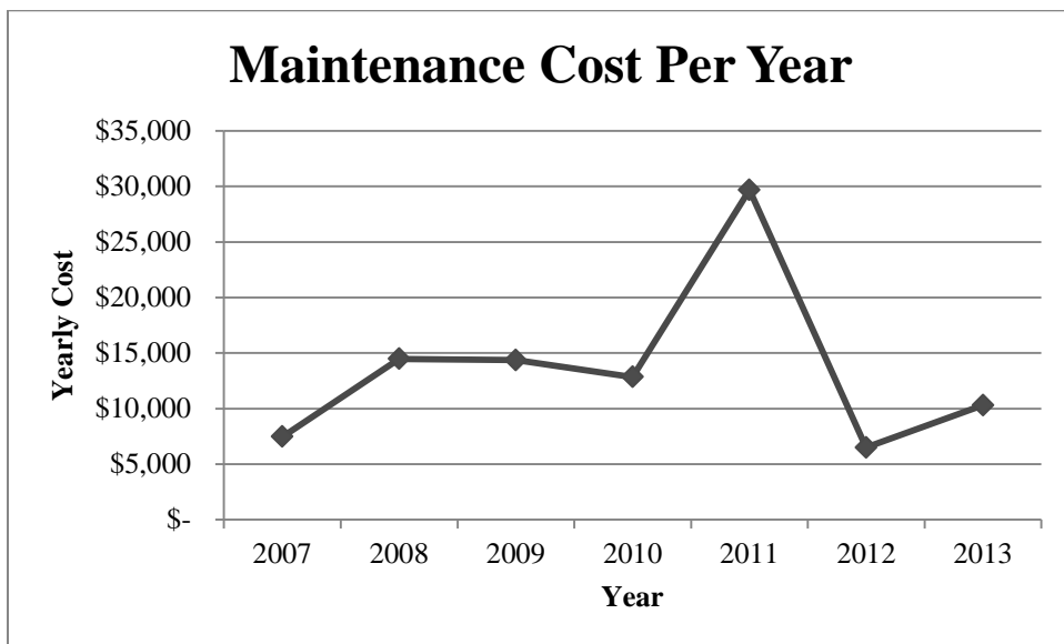
Figure 5- Actual yearly maintenance costs of one feller-buncher
