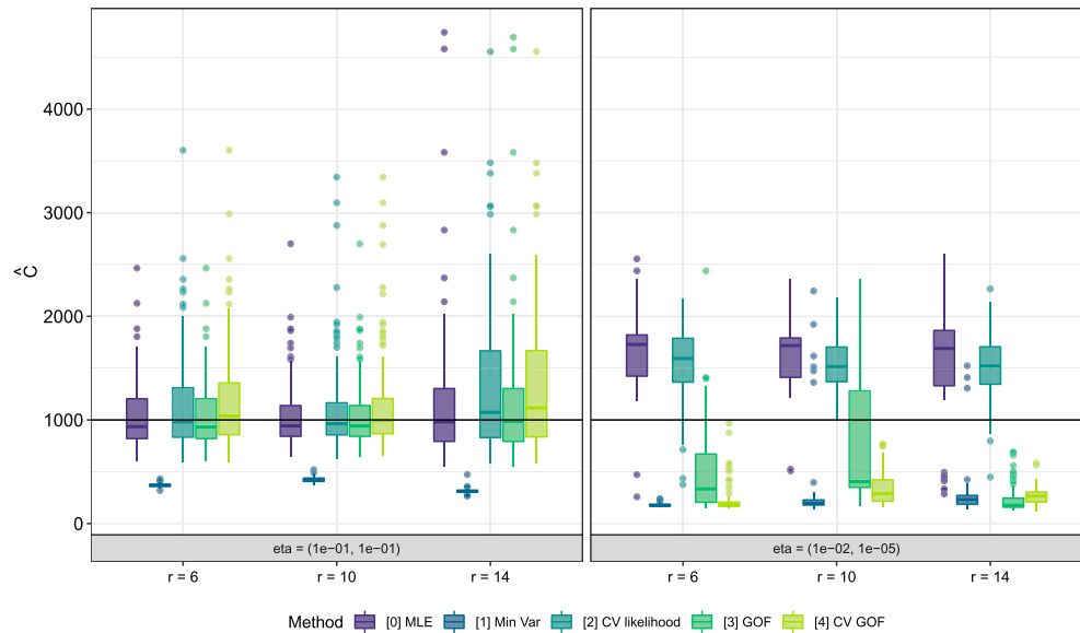
Figure 3. Simulation results for all proposed methods when \eta = (10^{-1}, 10^{-1}) , and when \eta = (10^{-2}, 10^{-5}) .
