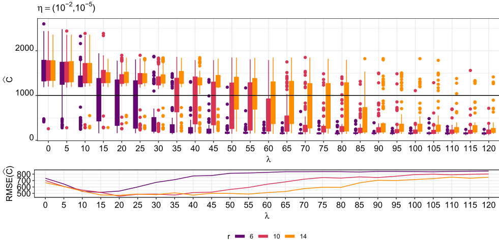
Figure 2. Estimates of C and their root-MSE over \lambda when \eta = (10^{-2}, 10^{-5}) and C = 1000 . Results are based on 100 simulations per \lambda .
