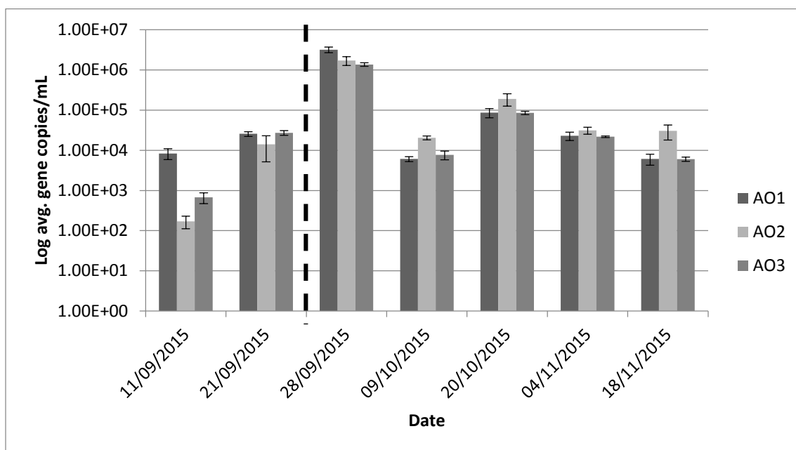
Figure 3.19: Relative abundance (target gene copies/mL) fluctuations of dsrB in the alkaline-only bioreactors throughout the experiment. The dashed line represents the treatment episode.
