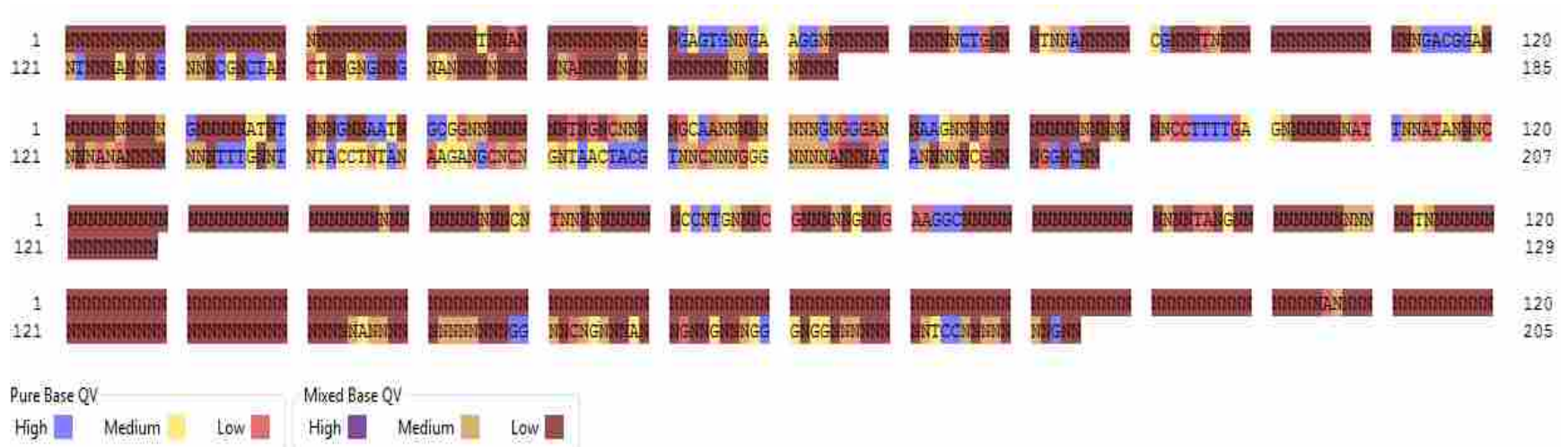
Figure A5: An example of three excised bands that were sent for sequencing. Although some base pairs were revealed, the purity of the product sent was not high enough. Therefore, band sequences came back with mixed base pairs (N).
