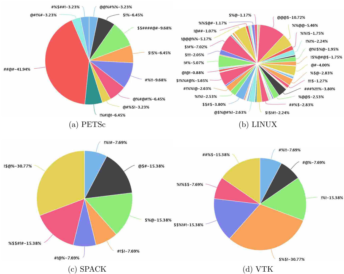
FIGURE 7. Profane words.
