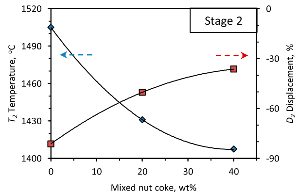
Figure 7. Effect of nut coke addition on the second stage bed characteristics temperature ( T_2 ) and contraction ( D_2 ).
