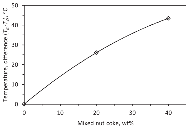
Figure 13. Effect of nut addition on the temperature difference between individual burden melting ( T_2 ) and bed melting temperature ( T_m ).
