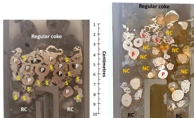
(a). Ferrous bed without nut coke, quenched at 1505 °C
