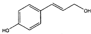
p-Coumaryl alcohol
