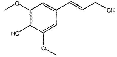
Sinapyl alcohol
