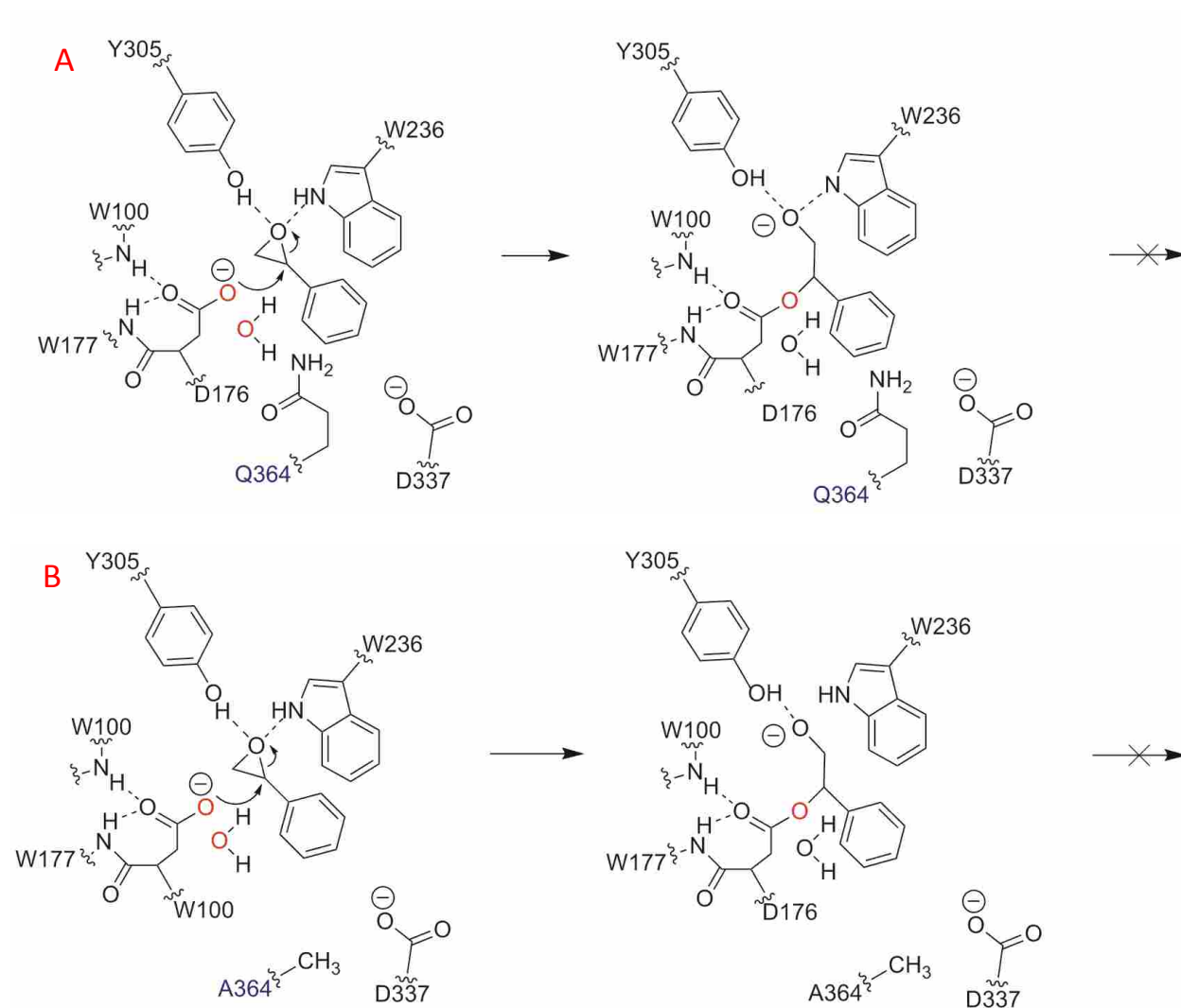
Figure 15. Proposed mechanism for styrene oxide hydrolysis by (A) SghF-H364Q and (B) SghF-H364A.
