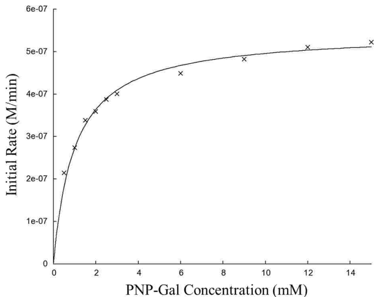
Figure 25. Michaelis-Menten plot of BT2857 expressed in Tuner(DE3)pLyss cells to confirm galactosidase activity with PNP-Gal: From the equation of the curve, the Michaelis-Menten variables were calculated where V_{\max} = 5.453e-7 \pm 1.105e-8 M/min, K_M = 1 \pm 0.0832 mM, and k_{\text{cat}} = 1.704e-3 s -1 . Curve produced using the online curve-fitting program ‘ K_M V_{\max} Tool Kit’ found on http://ic50.tk/kmvmax.html .
