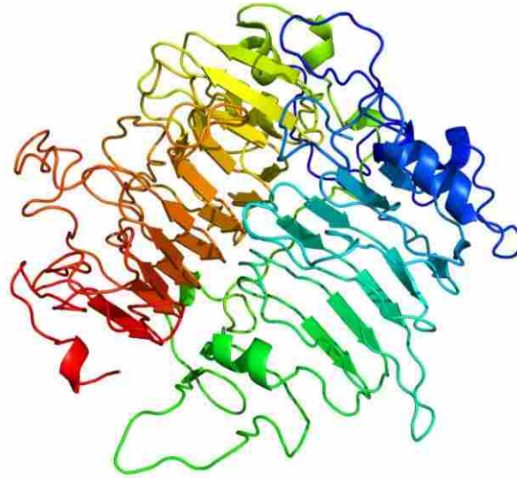
Figure 11. Phyre 2 predicted model of SCO6594 based on sequence homology with a beta-1,3-glucanase from Phanerochaete chrysosporium : The template sequence demonstrated 100.0% confidence and 95% coverage to the input sequence. The predicted model comprises of parallel beta-strands. Residues S12-V594 are modelled [3].
