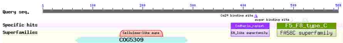
Figure 12. Basic local alignment search tool (BLAST) search of SCO6596: Results indicate predicted domains of a cellulase-like superfamily on the N-terminus, and cadherin repeat and F5/8 type C domain towards the C-terminus [8].
