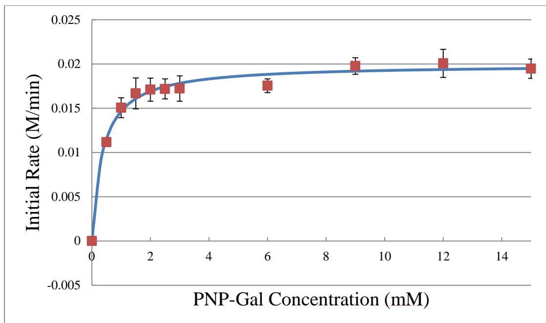
Figure 22. Michaelis-Menten plot of BT2857 kinetic activity with PNP-Gal: From the equation of the curve, the Michaelis-Menten variable were calculated where V_{\max} = 0.01994\text{M/min} , K_M = 0.3660\text{mM} , and k_{\text{cat}} = 6645\text{ s}^{-1} . Data points were produced from a set of triplicates.
