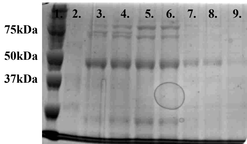
Figure 24. SDS-PAGE gel depicting the attempted purification of BT2857 (expressed in Tuner(DE3)pLyss cells) using anion-exchange chromatography: 12% SDS-PAGE gel loaded with elution fractions under the peak (chromatogram not shown)
