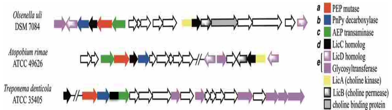
Figure 4. Phosphonate gene clusters from representative bacteria, with genes colour coded according to annotation. Lower case letters beside the colour codes in the legend correspond to the letters that label the enzymatic steps in Figure 3.
