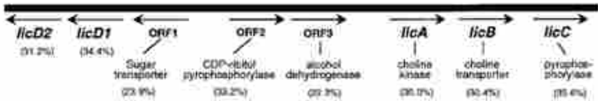
Figure 6. Gene cluster of S. pneumoniae and potential function of the gene products based on sequence similarity are listed 28
