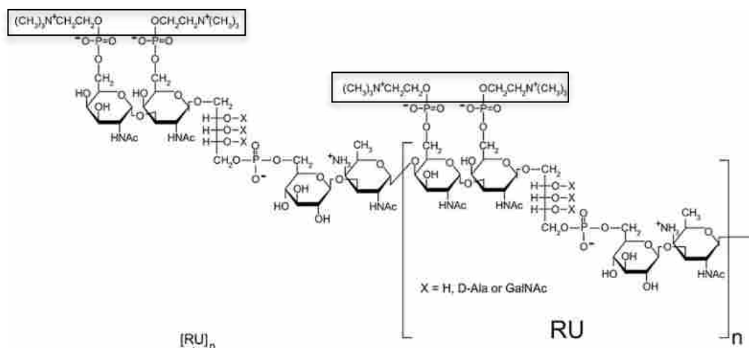
Figure 5. Teichoic acid of Streptococcus pneumoniae with P-Cho incorporated into it. P-Cho is highlighted in the box 26 .
