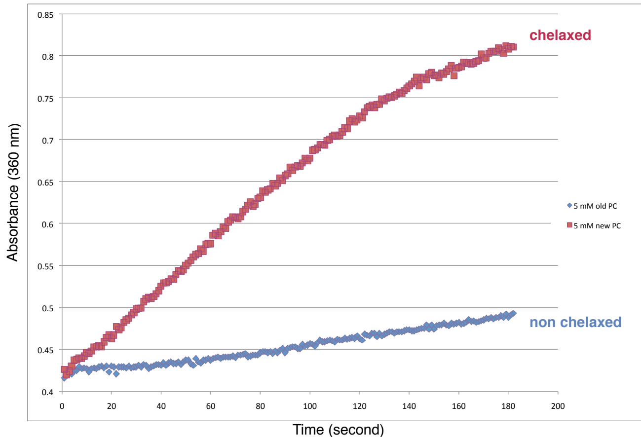
Figure 37. Pyrophosphate release from Spn-LicC enzyme with 5 mM chelaxed and non chelaxed phosphocholine.
