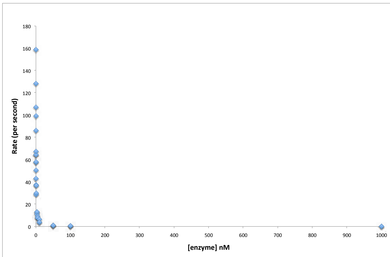
Figure 38. Spn-LicC activity assay with 0.1 mM phosphocholine and various concentrations of enzyme.
