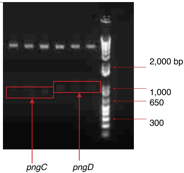
Figure 22. Oul- pngC pET29 and Oul- pngD pET29 construct digests with Nde I and Xho I restriction enzymes. Lanes 1-3 show LicC construct digest at 790 bp and Lanes 4-6 show LicD construct digest at 930 bp. Lane 7 shows molecular weight ladder.
