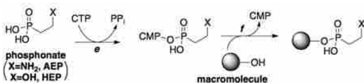
Figure 9. Proposed tailoring steps to add a phosphonate to a macromolecule with the following enzymes: e , cytidylyltransferase; f , phosphotransferase or glycosyltransferase.
