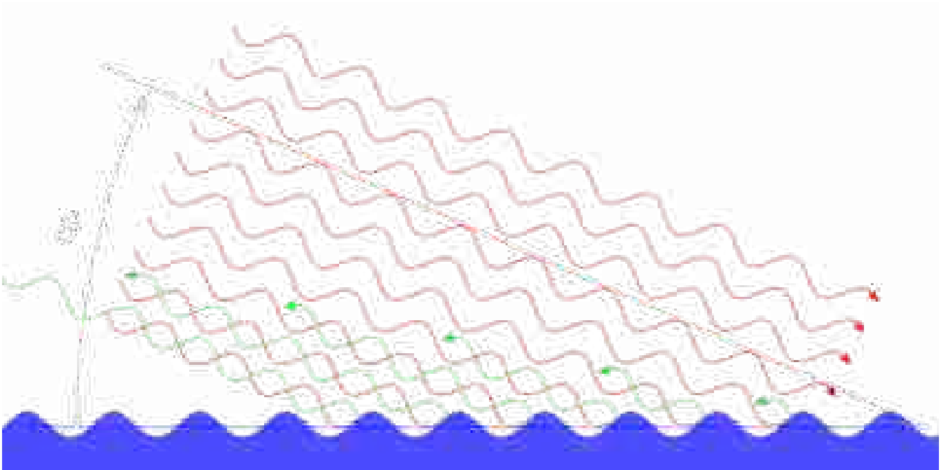
Figure 2.1: Bragg Scattering by Christian Wolff
