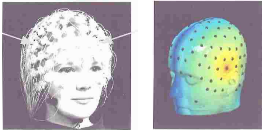
FIGURE 5.1: EIT measurements, small alternating current injected into pair of electrodes and the response is measured at the rest of the electrodes. Data acquisition set up (left) and the computational model (right).
