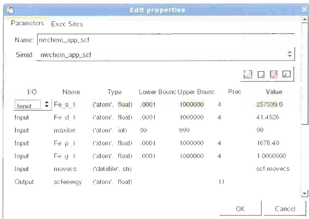
FIGURE 8.1: NWChem simulation specification.
