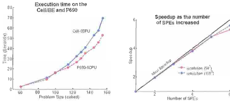
FIGURE 4.7: Performance of the forward solver on the Cell Be. Comparison with a shared memory implementation (left) and Speedup curve (right).
