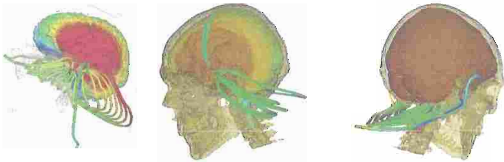
FIGURE 4.4: Current and potential distributions due to a current dipole source in the cortex; holes in the skull allow more current to flow through the skull and reach the scalp, which increases the effective conductivity of the skull.
