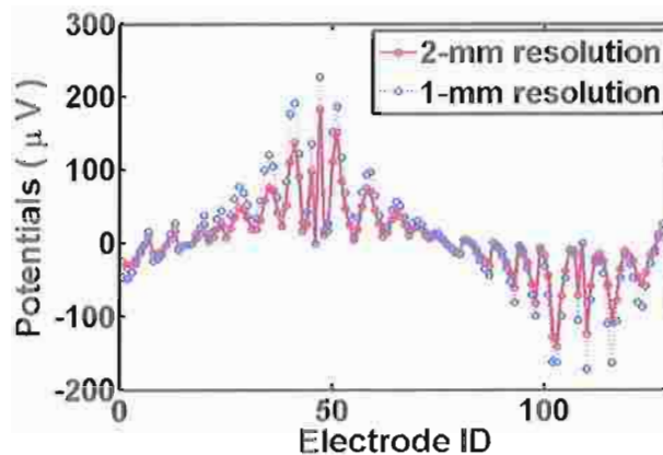
FIGURE 8.7: The potentials at the electrodes using 1mm resolution geometry vs. 2mm resolution.
