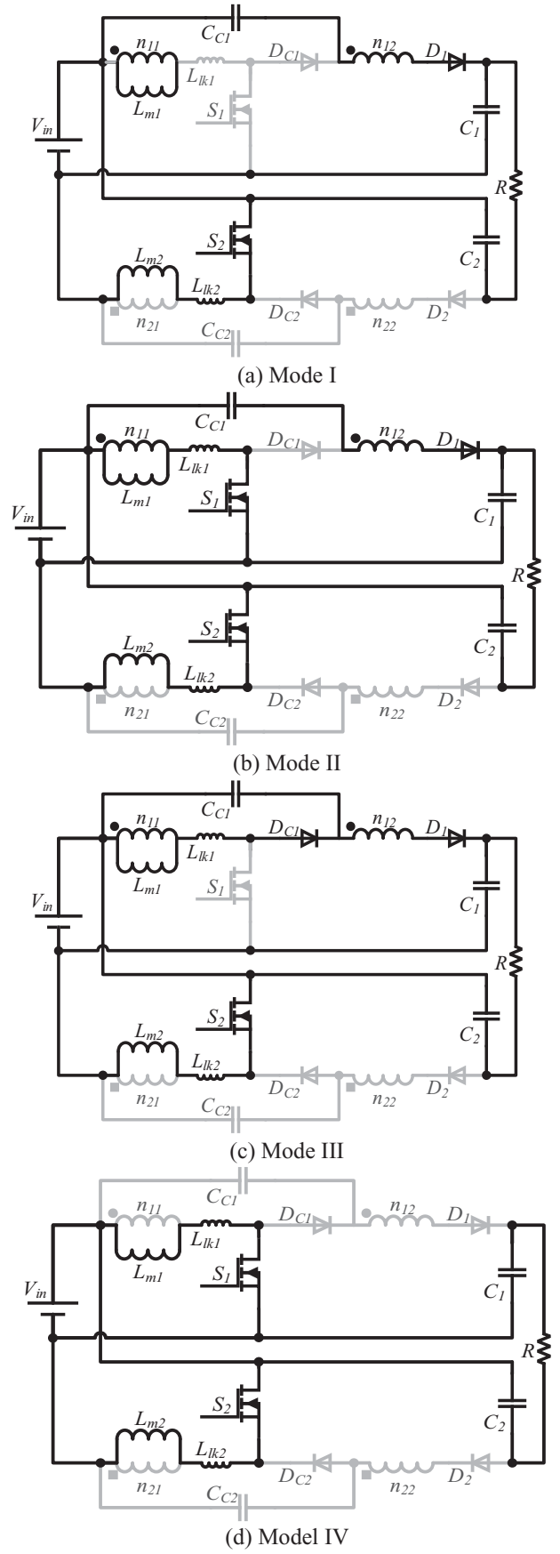
Figure 3. Equivalent circuit of the operating modes.
