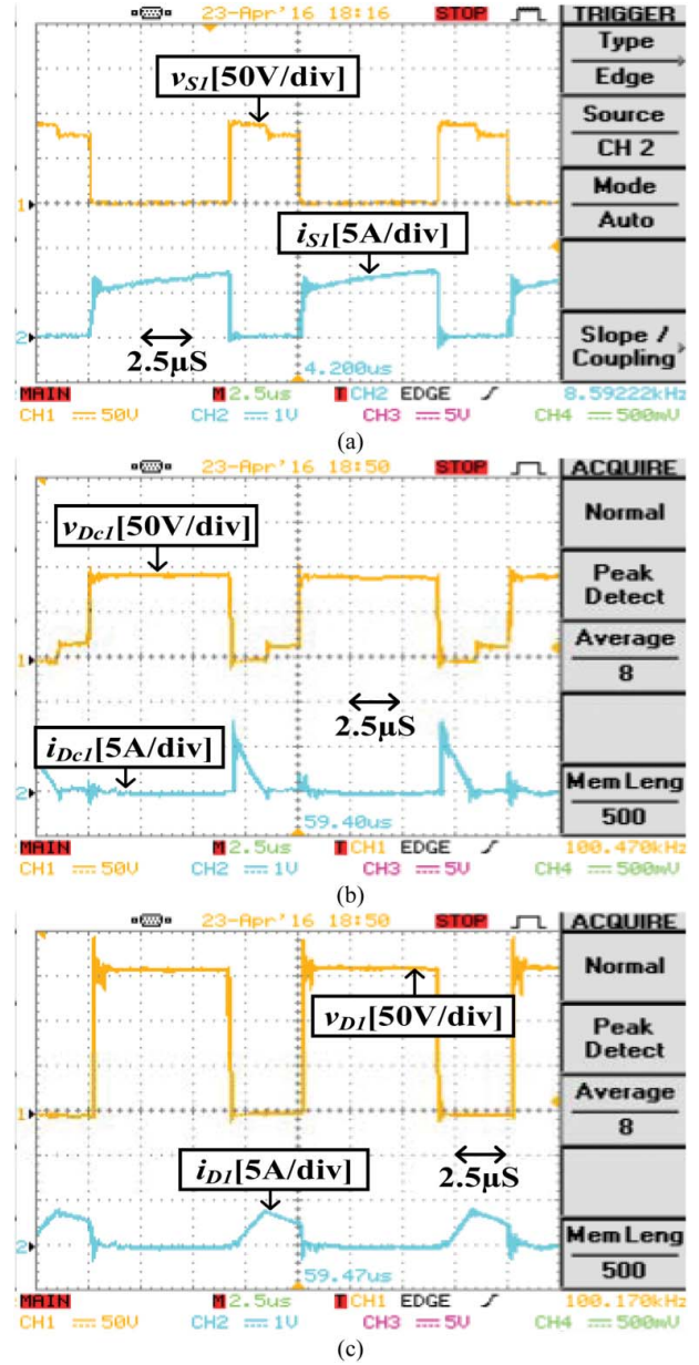
Figure 9. Experimental waveforms of the proposed converter: (a) v_{ds1} , i_{ds1} ; (b) v_{Dc1} , i_{Dc1} ; (c) v_{D1} , i_{D1} .
