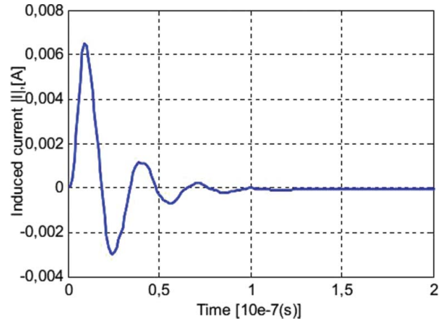
Figure 6. Transient current induced in the feet due to the bi-exponential pulse exposure.
