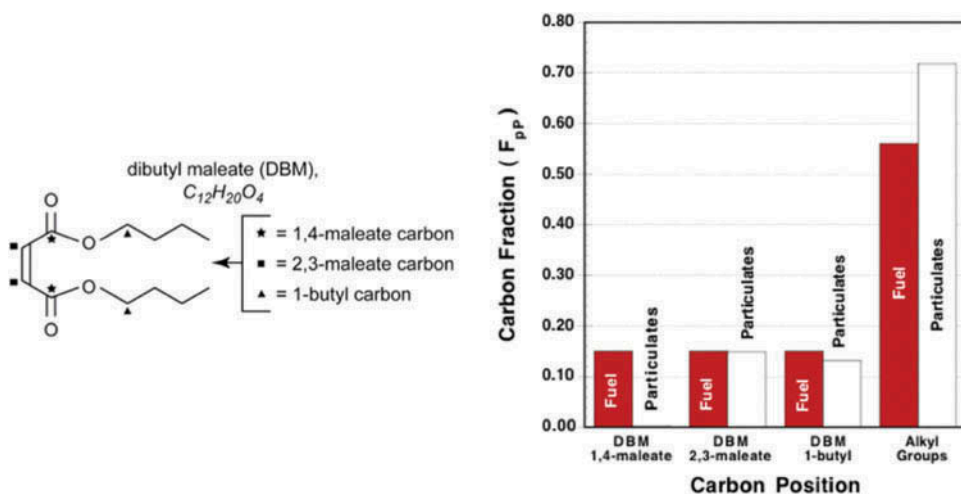
Figure 1. Molecular structure of dibutyl maleate (DBM) and positions of ^{14}\text{C} labels, and chart showing the relative contributions of the labeled positions to particulate matter. [Reprinted from Buchholz et al. (2004) with permission from SAE International.]
