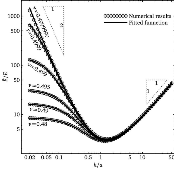
Figure 6. Comparison of the fitted analytical function (solid lines) with finite element results (circles) for the equivalent modulus for various Poisson's ratios.
