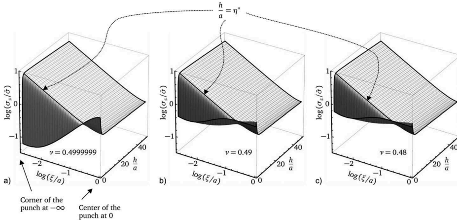
Figure 9. Normal stress, \sigma_z/\bar{\sigma} , along the interface (logarithmic scales base 10) between the rigid punch and the elastic layer as a function of layer confinement h/a for Poisson's ratio (a) 0.4999999, (b) 0.49, and (c) 0.48. The coordinate \xi corresponds to the distance from the perimeter toward the center of the punch (see Figure 1). The solid line, labeled with \eta^* , highlights the stress distribution at the critical confinement ratio h/a = \eta^* (see Table 2).
