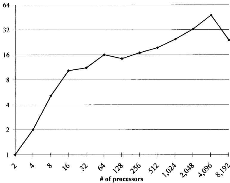
FIGURE 68. 524k SCA#2: Speedup.
