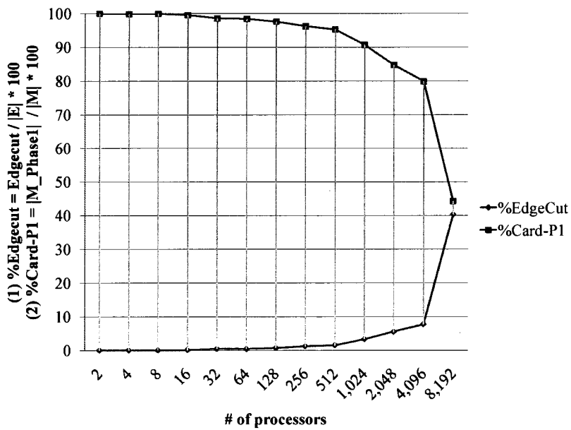
FIGURE 69. 524k SCA#2: Cardinality after Phase-1.
