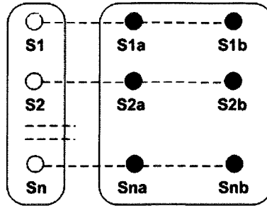
FIGURE 31. Intuition for proof of \frac{2}{3} -approx algorithm GLOBALTWO THIRD. For each failed S vertex, Algorithm GLOBALTWO THIRD will match two S vertices that are at least as heavy as the failed vertex. Note that the association of matched vertices with failed vertices is dynamic. The figure is representative of a state at a particular step of execution.
