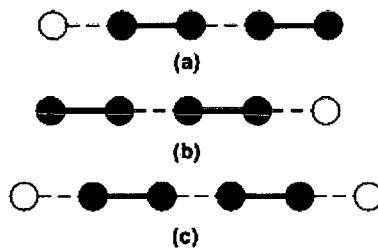
FIGURE 7. Types of paths. Matched edges are represented with bold lines and matched vertices are colored black. (a) An alternating path starting with an unmatched vertex, (b) an alternating path starting with a matched vertex, and (c) an augmenting path.
