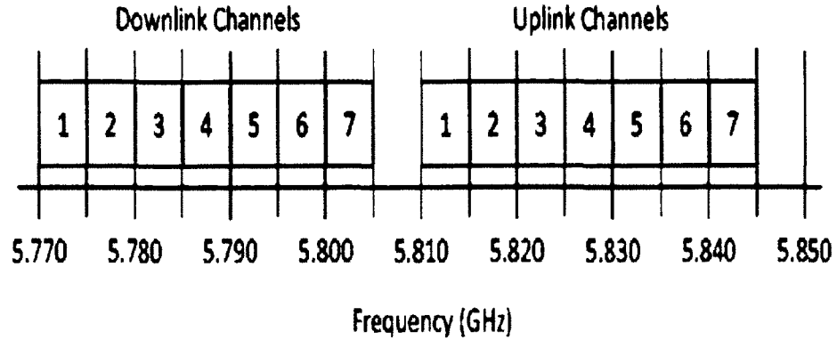
FIG. 16: Japan DSRC channels
