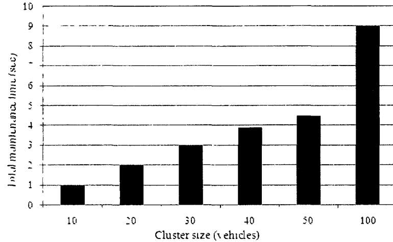
FIG. 26: Impact of cluster size on cluster maintenance time
