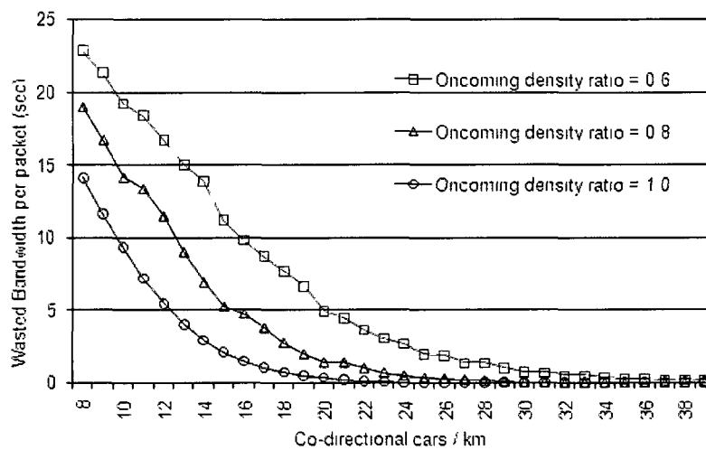
FIG. 31: DPP Overhead per packet
