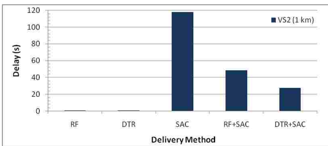
Figure 24. Average message delay from VS_2 with different delivery methods.
