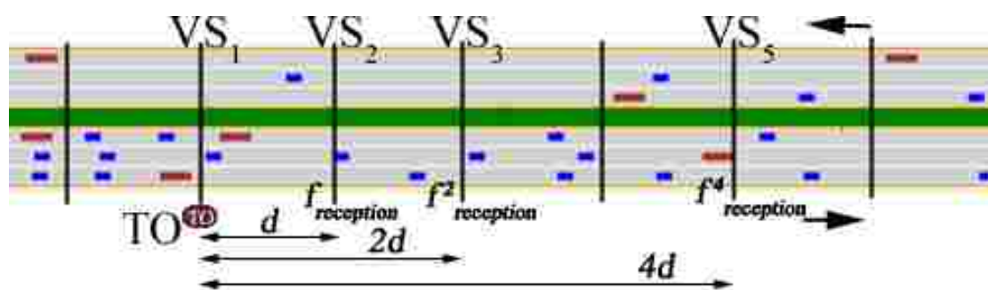
Figure 16. Relationship between distance d and probability of message reception
