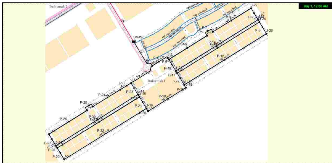
Figure 5.2: Layout of EPANET junctions and pipes
