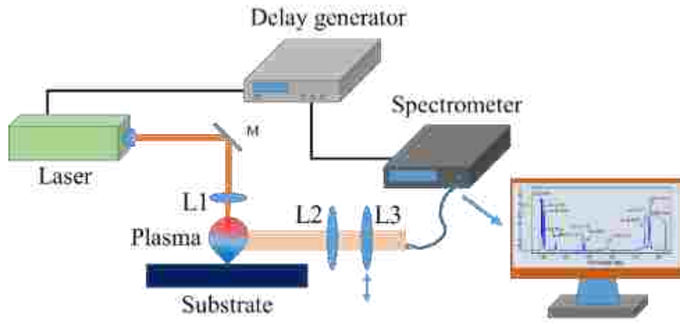
Fig. 2.4 Experimental setup of optical emission spectroscopy. The image of the laser plasma is created by combination of L2 and L2 lens. Delay generator is used to determine the time-resolved optical spectra.
