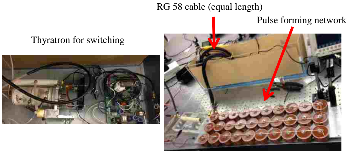
Fig. 3.10 The construction of the pulse forming network with thyatron switching and variable resistance.
