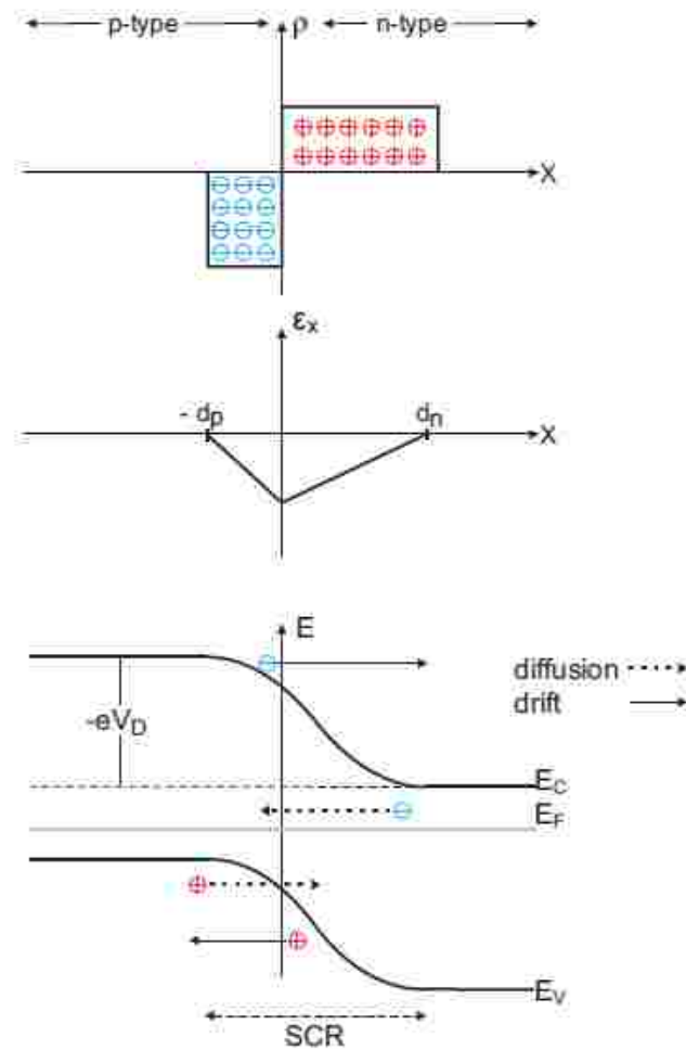
Figure 1.2: Schematic of a p-n junction illustrating the space charge distribution, electric field distribution and energy band diagram [8]
