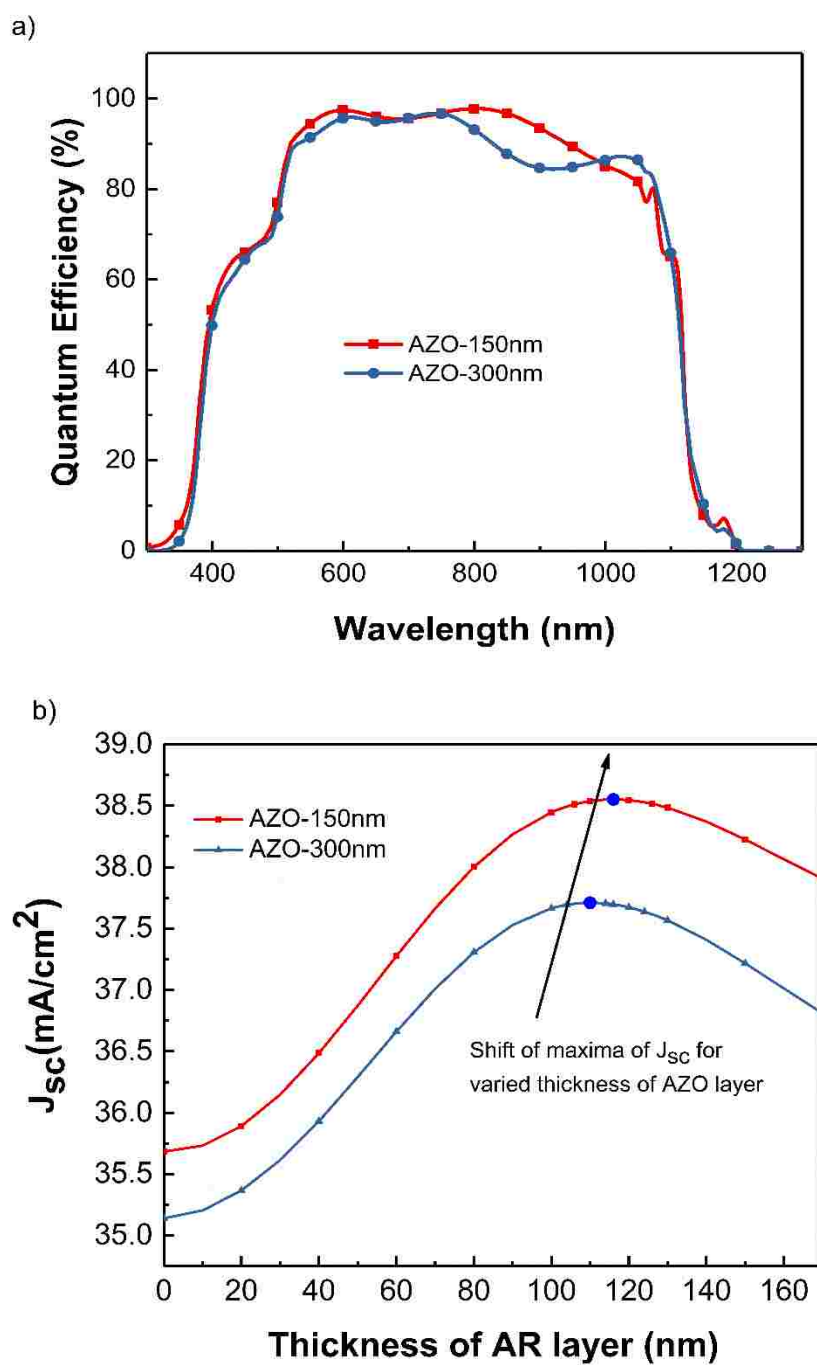
Figure 3. 14:a) Simulated variation of QE with varied thickness of AZO layer for a fixed value of \text{MgF}_2 (110 nm), and b) Simulated J_{sc} as a function of \text{MgF}_2 thickness for various thickness of AZO layer.
