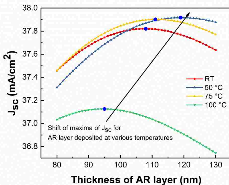
Figure 3.21: Simulation of the variation of J_{SC} for CIGS devices with varied thickness of MgF_2 layer deposited at different T_{SS} .
