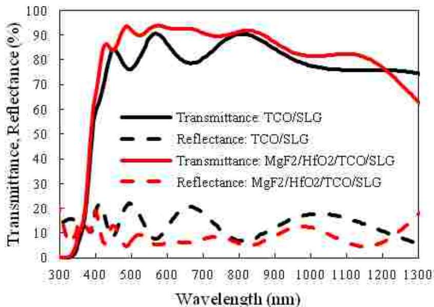
Figure 5. 5: Measured reflectance and transmittance spectra of a standard TCO structure on SLG before and after deposition of a 2-layer MgF 2 /HfO 2 AR coating
