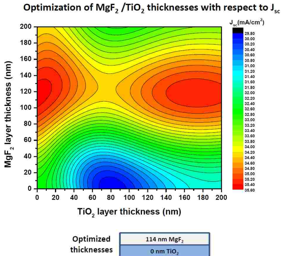
Figure 5.2: Predicted variation of J_{sc} with MgF 2 /TiO 2 thicknesses: J_{sc} - 35.5 mA/cm 2
