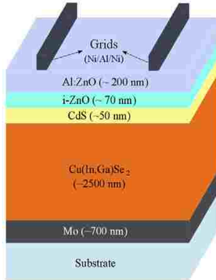
Figure 1.1: Illustration of the CIGS device structure
