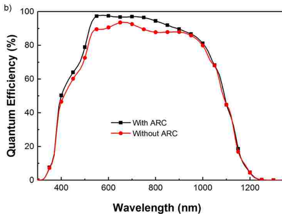
Figure 3. 7: Comparison of measured J-V curves and QE spectra obtained for CIGS solar cells with and without AR coating.
