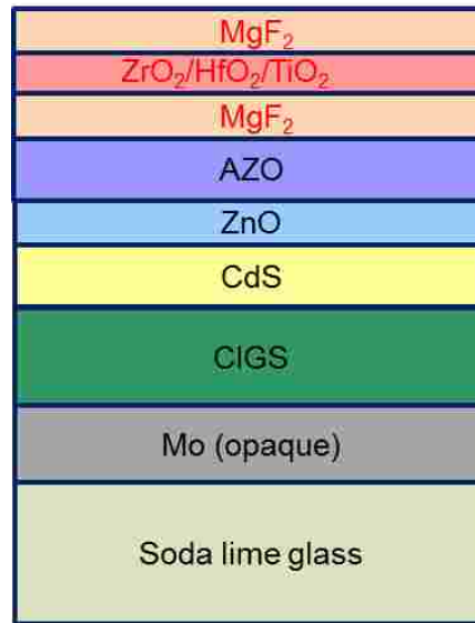
Figure 5. 9: Schematic diagram of ultra-thin CIGS solar cell with 3-layer ARC.
