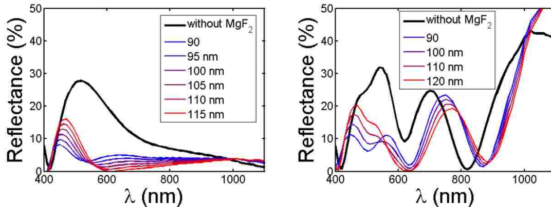
Figure 4. 6: Simulated reflectance from a regular CIGS device (left) and ultra-thin CIGS device with \text{MgF}_2 AR layer of varied thickness
