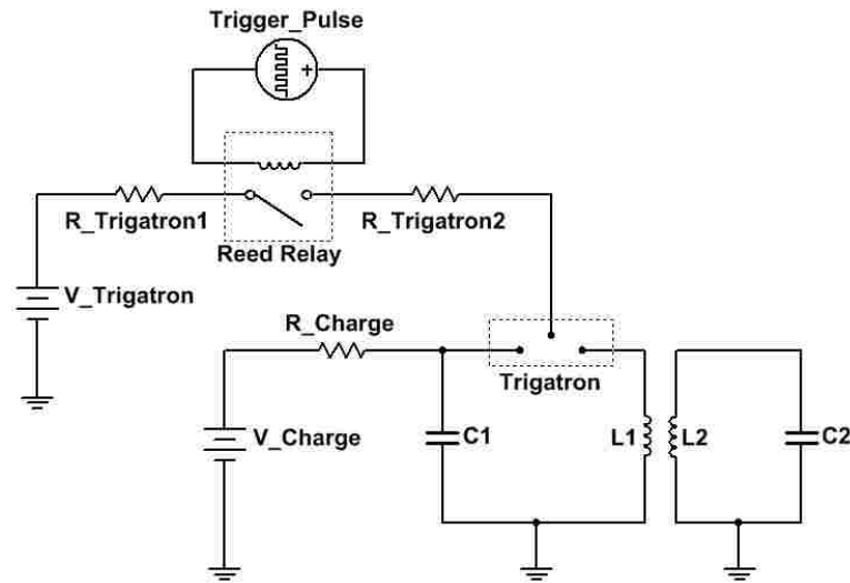
Fig. 42 Integration of a trigatron into the DRPT system
