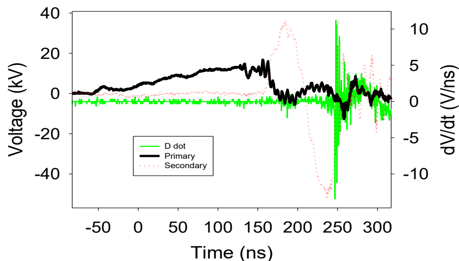
Fig. 45 Measured voltages of the combined system. After charging the primary capacitor (black), the first spark gap closes initiating the transformer response (red). The peaking switch closes near the maximum of the second voltage cycle, which is shown by the sudden drop in voltage in the secondary. This induces a fast transient in the D dot probe (green). [55]
