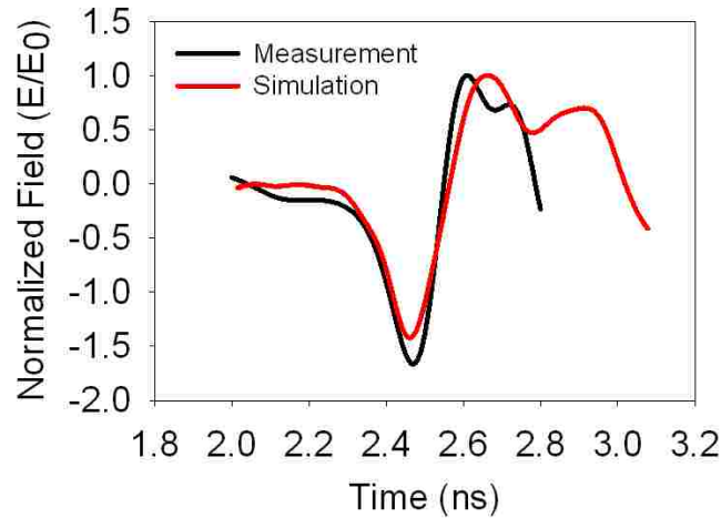
Fig. 11 Measured and simulated transients of the conical launching section [21]
