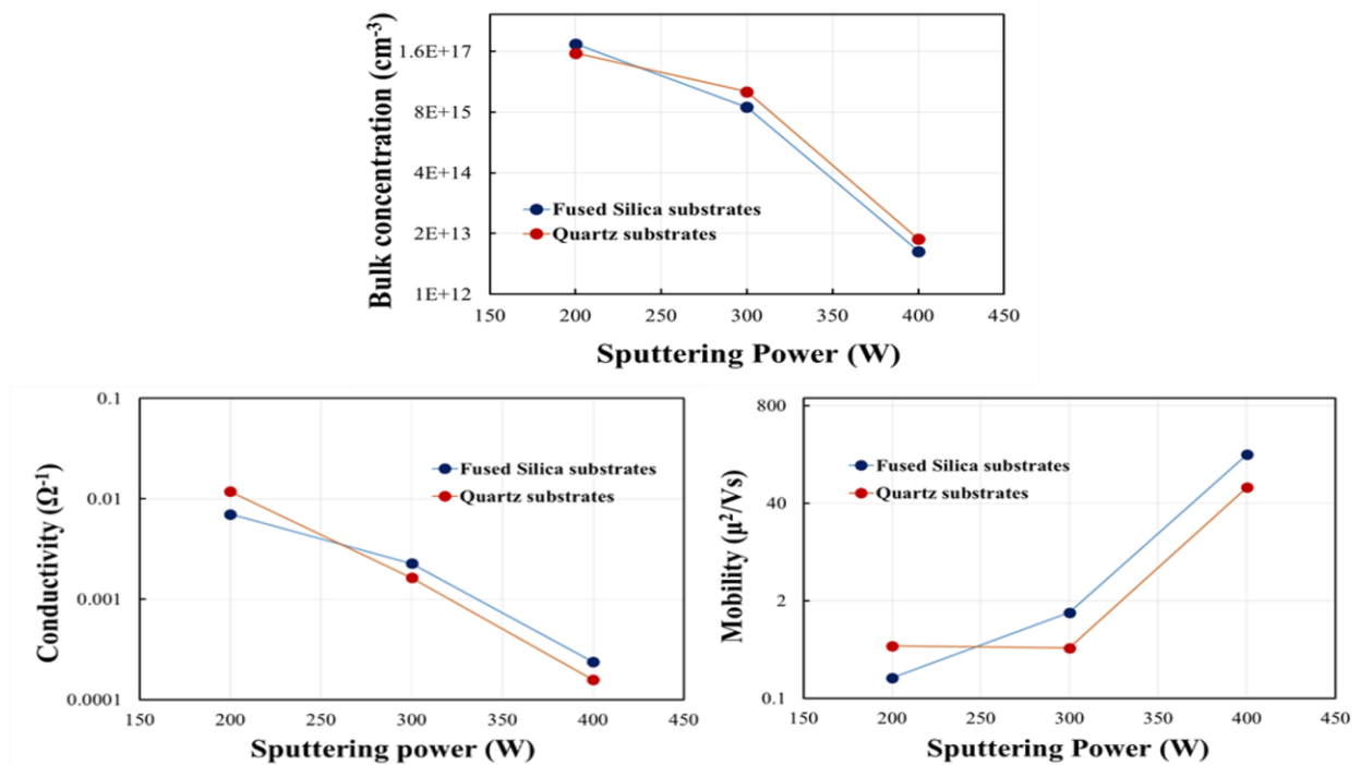
Fig. 3.8 Influence of sputtering power on electrical properties of the silicon films for different substrates
