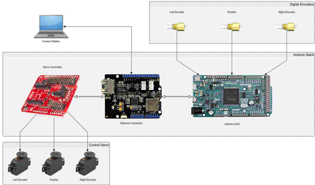
FIG. 20: Hardware Stack
