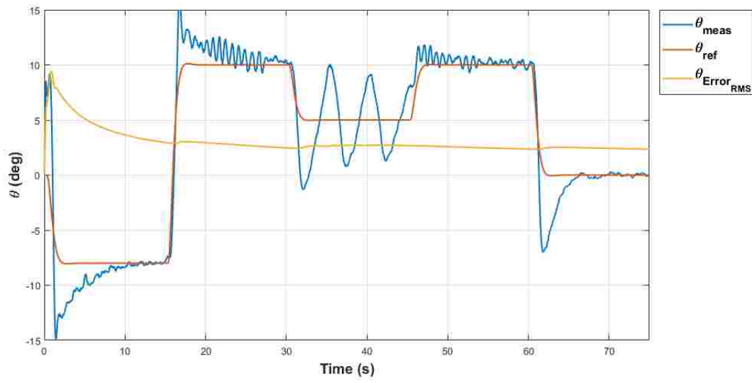
FIG. 27: LEX Aircraft Response to Doublet Input (Closed Loop)
