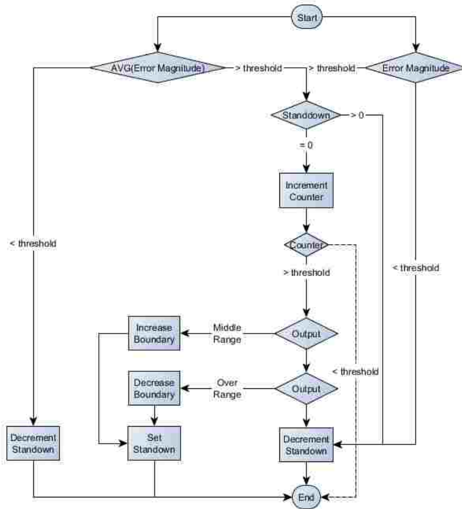
FIG. 29: Output Adaptation Algorithm
