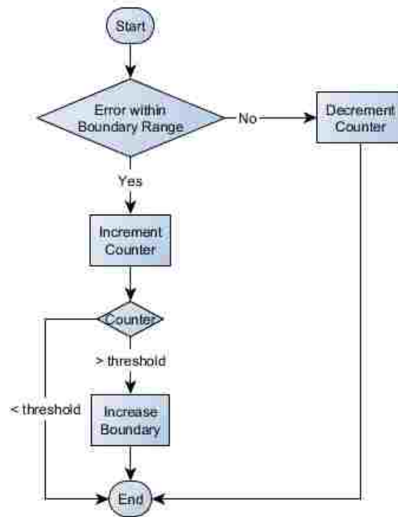
FIG. 28: Input Adaptation Algorithm
