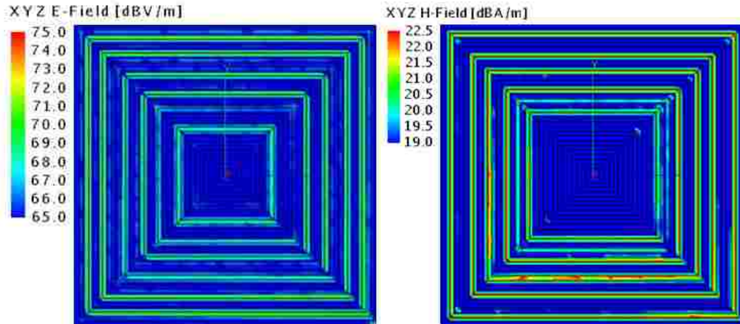
Fig. 23. E-field and H-field of 8-inch SansEC at primary resonance, 51 MHz [3], [14]
