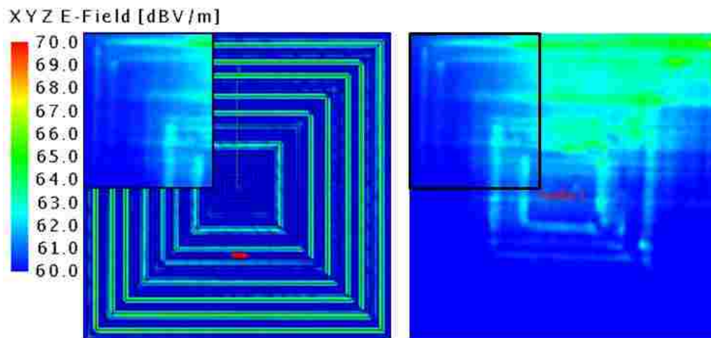
Fig. 28. 9-inch SansEC E-field at 52 MHz compared with IR image [3], [14]
