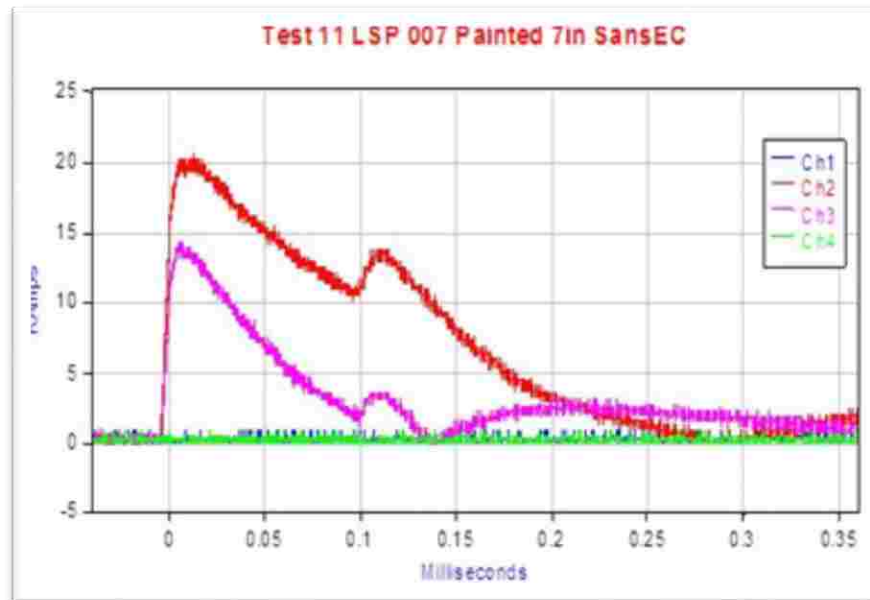
Fig. 14. Measured Electric Currents on 7-inch SansEC [3], [14]
