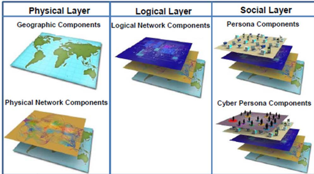
Figure 1 Cyber Domains
